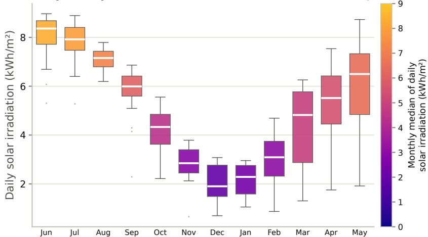
Konya: daily solar irradiation over the last 12 months (Jun 2025 - May 2026)
