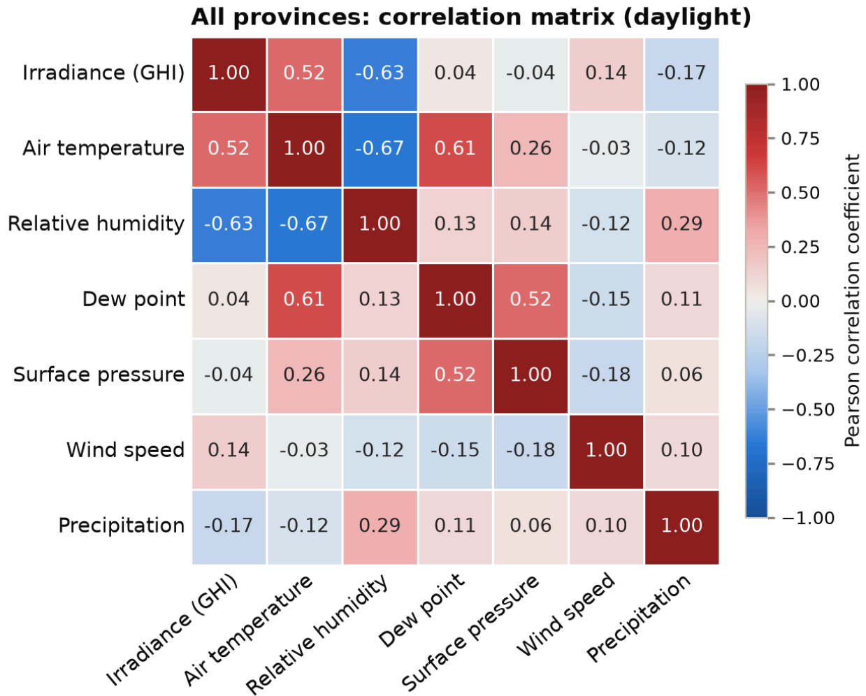
Figure 6. Correlation matrix of the target and the meteorological variables over daylight hours, pooled across sites.
