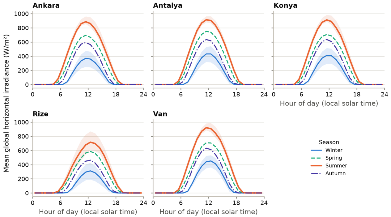
Mean daily cycle of irradiance by season (shaded: interquartile range across days)
