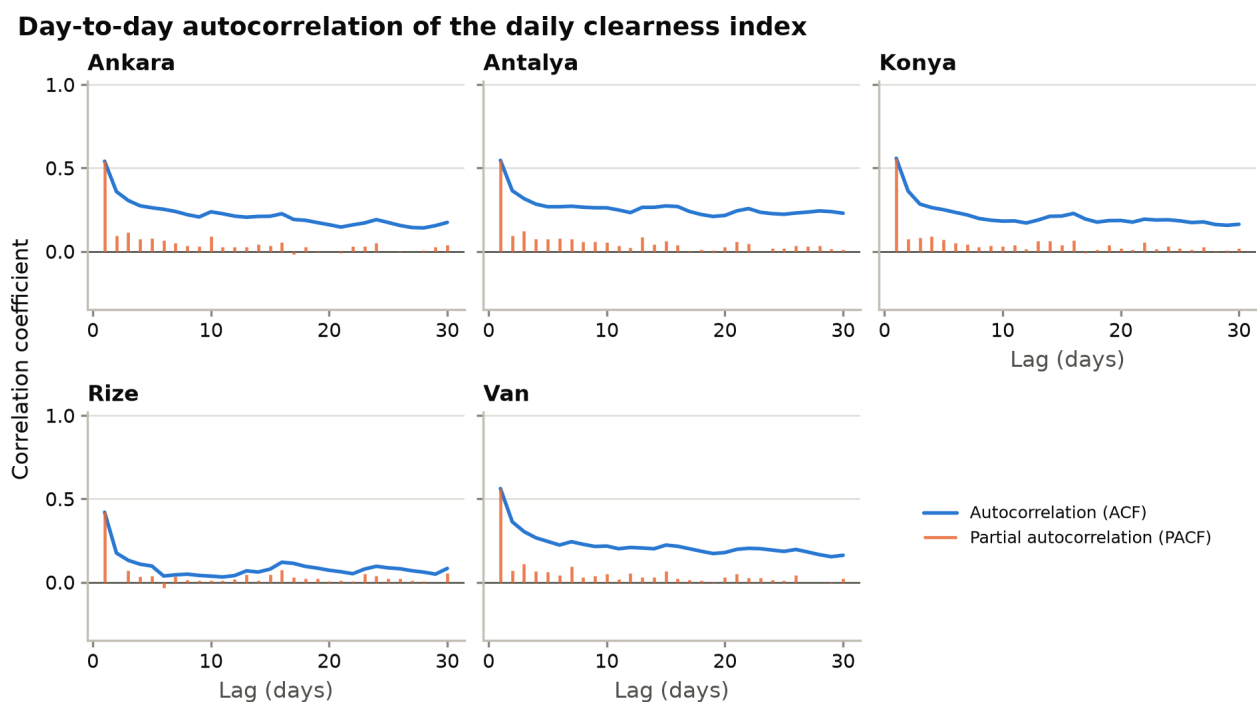
Figure 7b. Autocorrelation and partial autocorrelation of the clearness index at daily resolution, by site.
