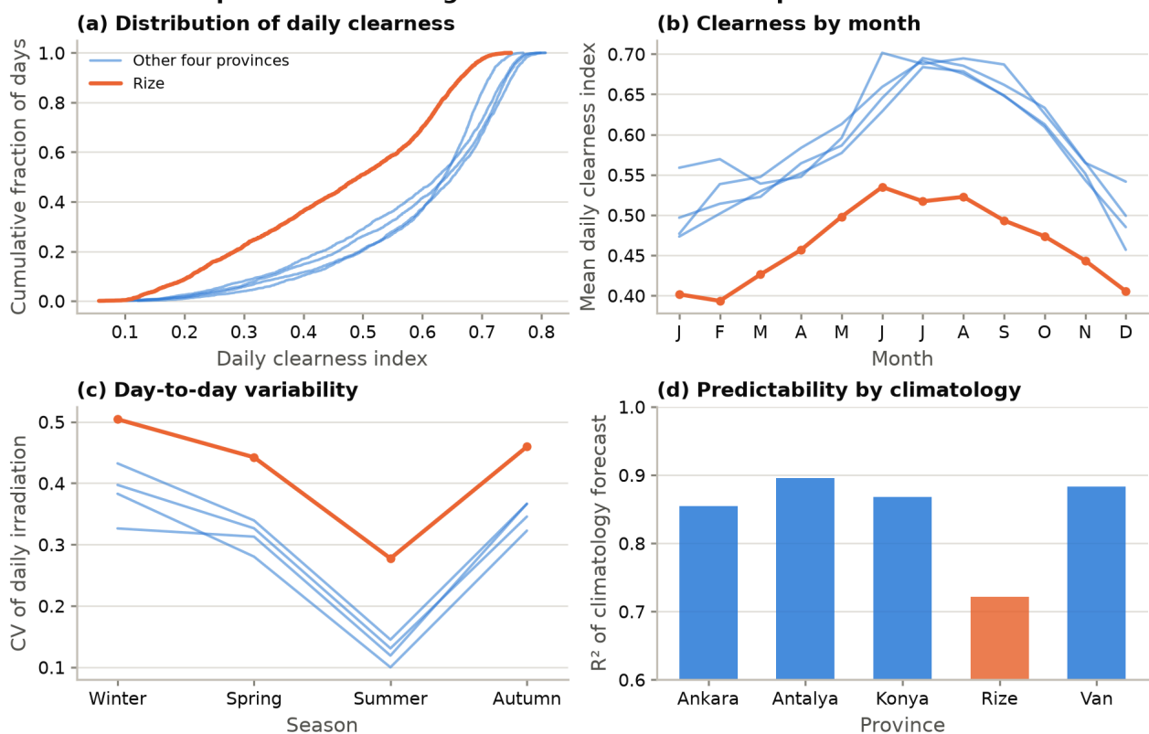
Figure 4. Radiative regime of Rize against the other four sites: cumulative distribution of the daily clearness index, the monthly clearness cycle, seasonal between-day variability, and the accuracy of the climatological reference forecast.
