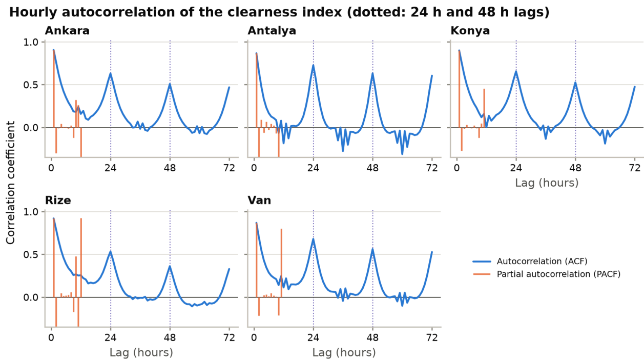
Figure 7a. Autocorrelation and partial autocorrelation of the clearness index at hourly resolution, by site. Dotted lines mark lags of 24 and 48 h.
