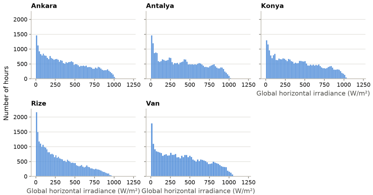
Figure 1. Distribution of hourly irradiance over daylight hours, by site.
