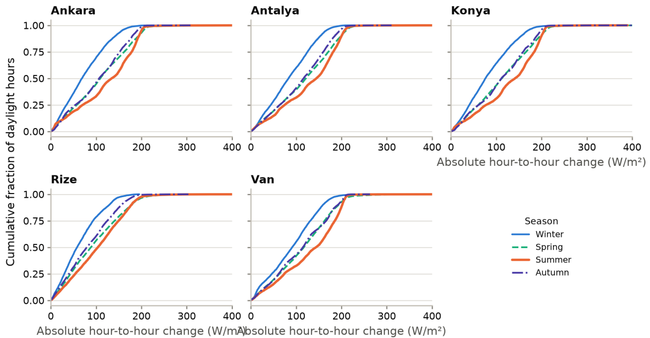
Cumulative distribution of hour-to-hour irradiance changes (daylight hours)
