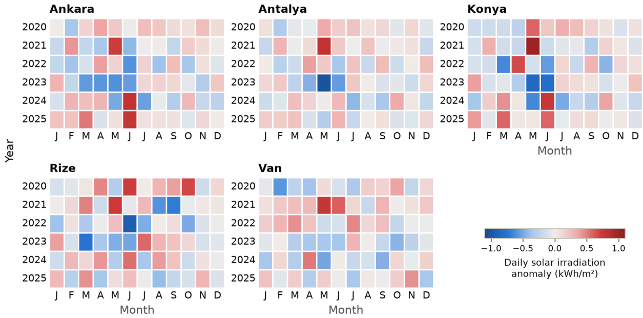
Figure 3. Month-by-year irradiance anomaly, expressed as the departure of each month from its six-year mean, by site.
