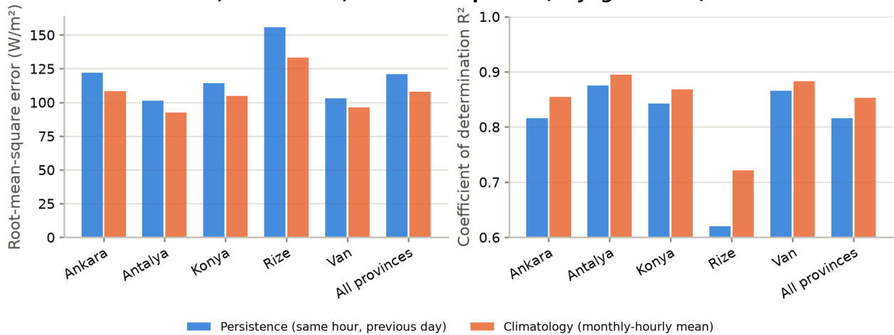
Reference forecasts, 24 h ahead, on the test period (daylight hours)
