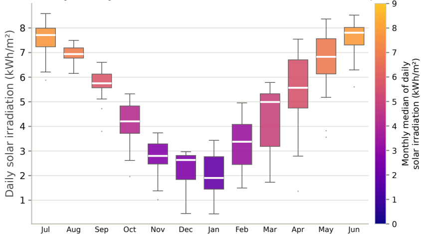
Antalya: daily solar irradiation over the last 12 months (Jul 2025 - Jun 2026)
