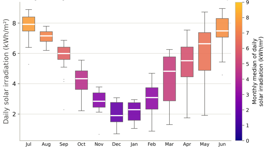
Konya: daily solar irradiation over the last 12 months (Jul 2025 - Jun 2026)
