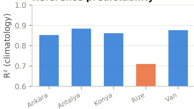
Reference predictability
