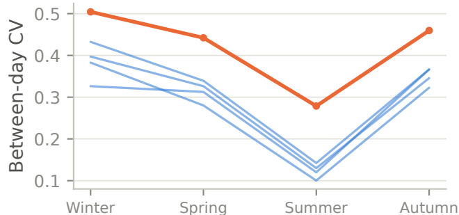
Seasonal variability
