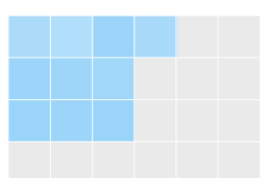
fixed_regressed
