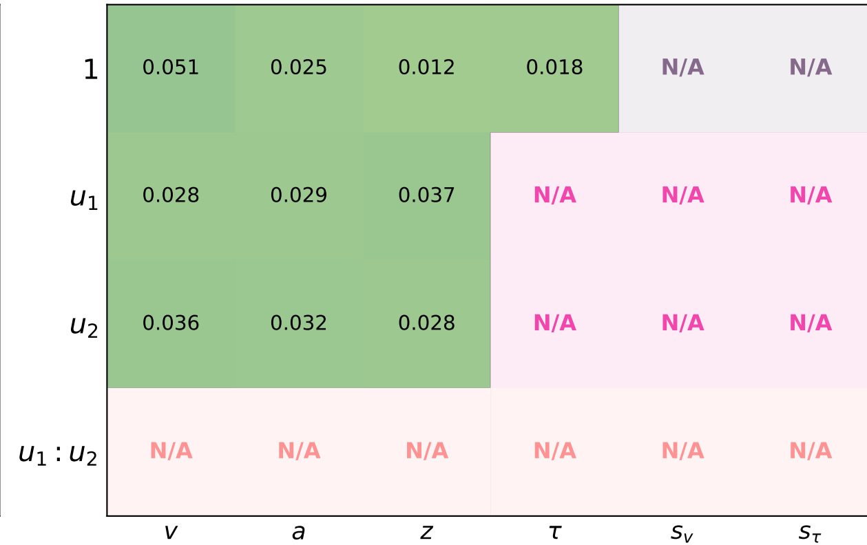
Calibration Error
