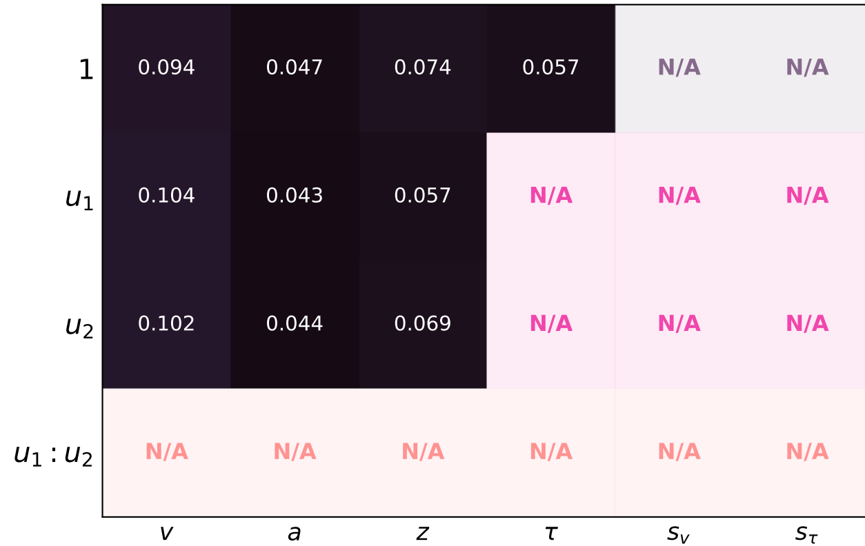
NRMSE
