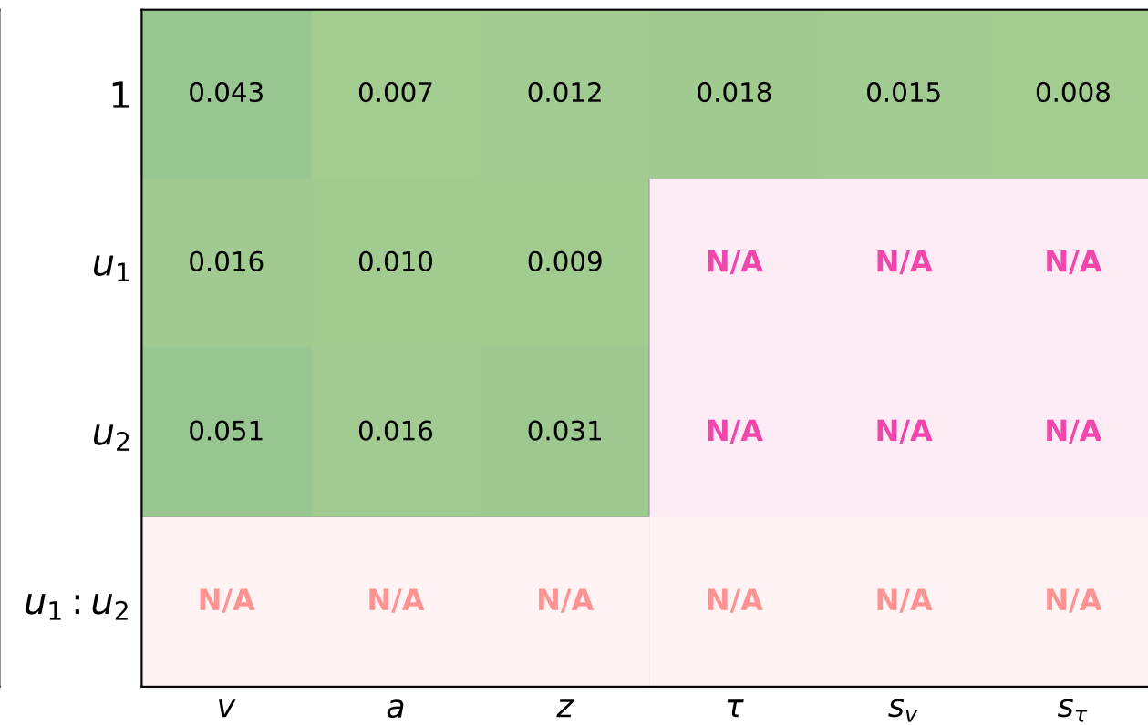
Calibration Error
