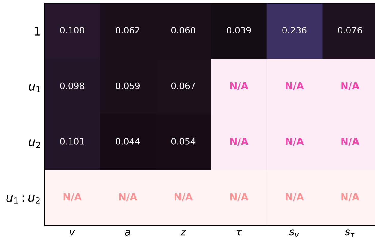
NRMSE
