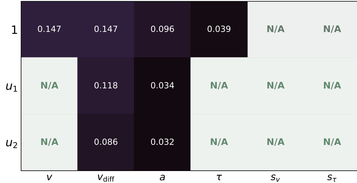
NRMSE
