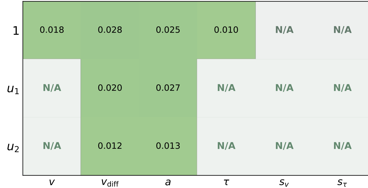
Calibration Error
