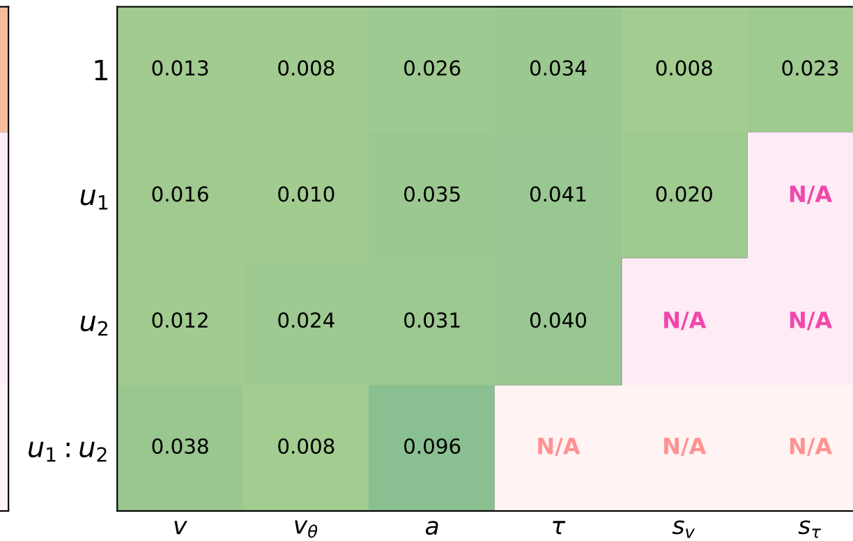
Calibration Error
