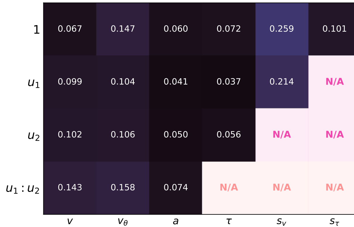
NRMSE
