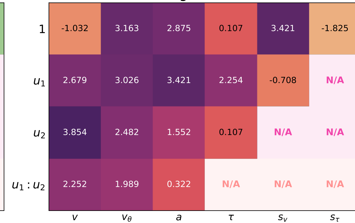
Log Gamma
