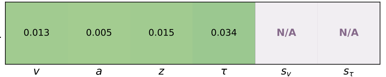
Calibration Error
