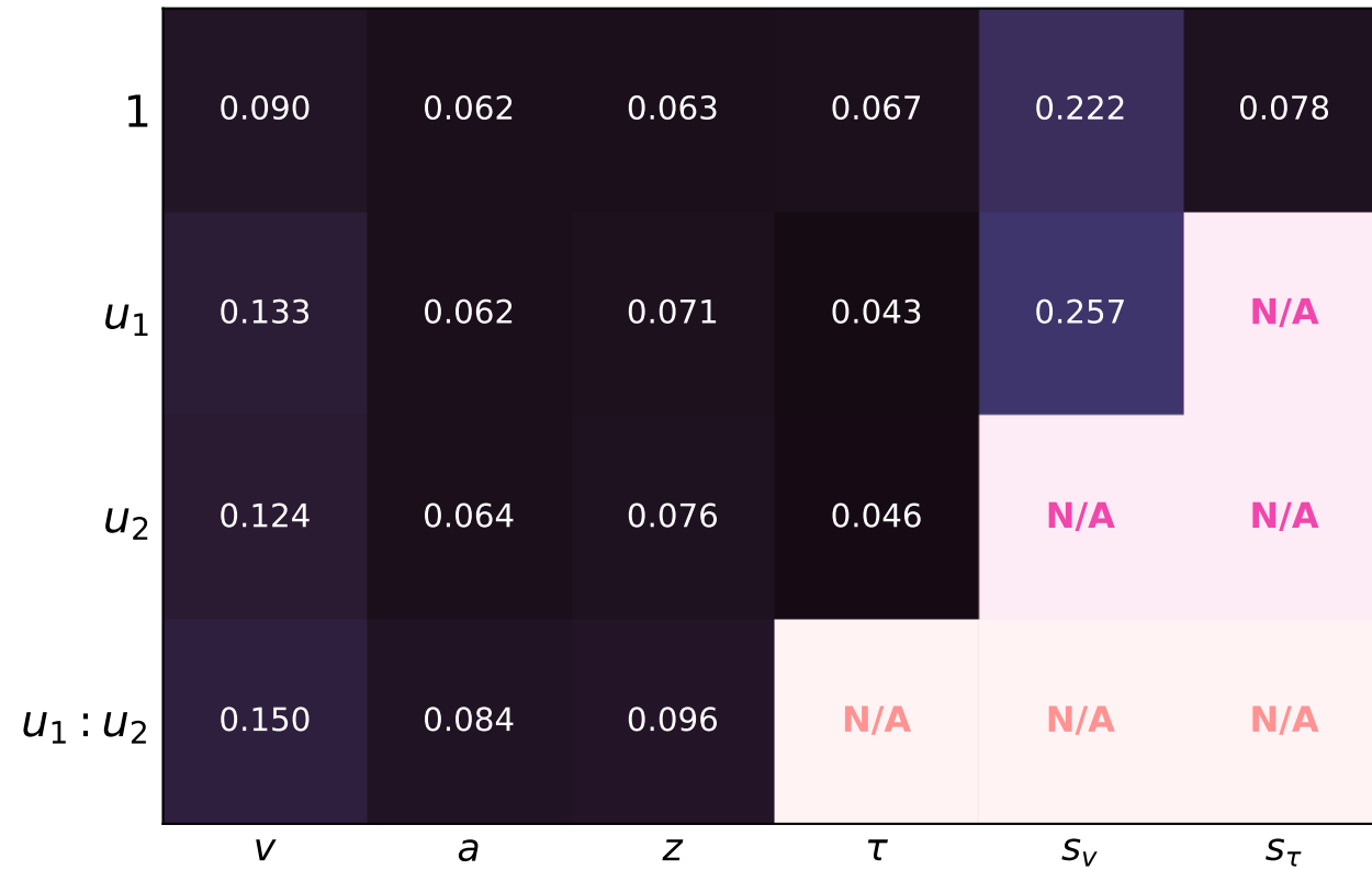
NRMSE
