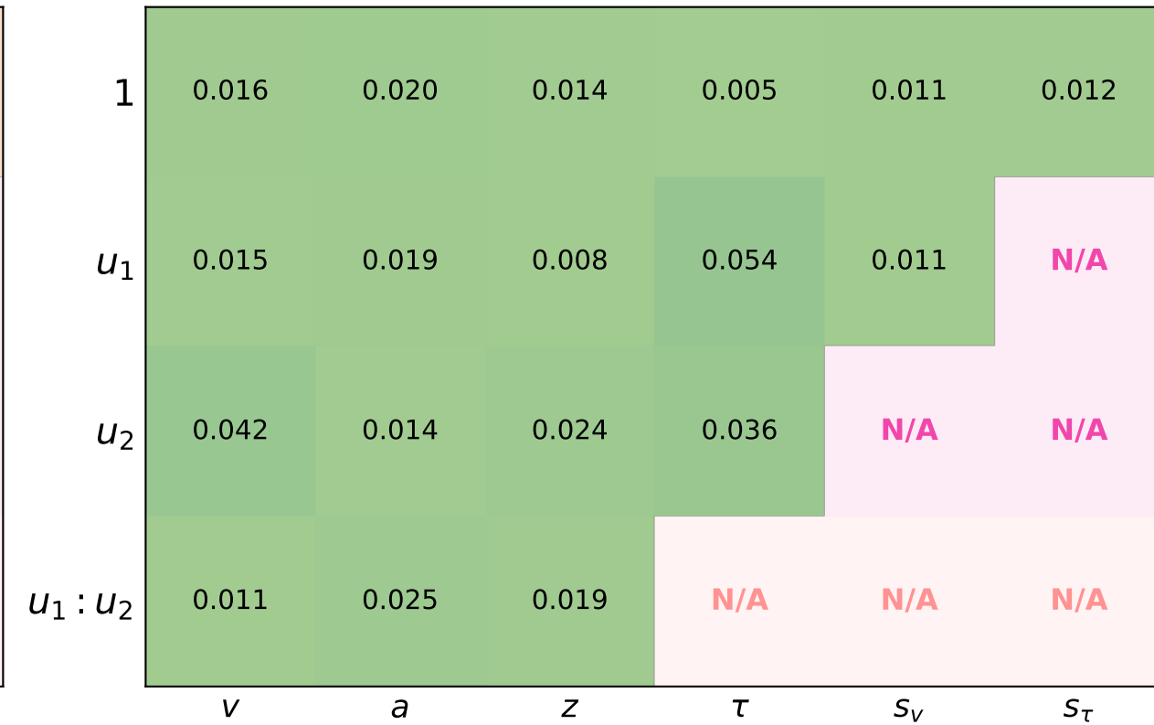
Calibration Error
