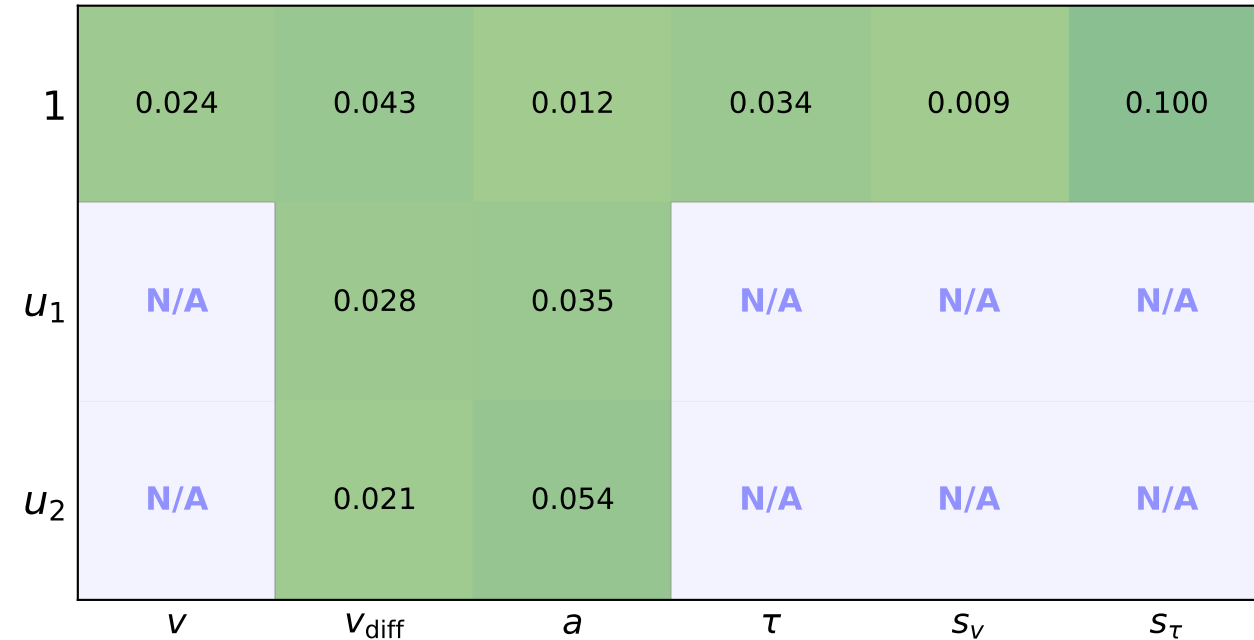
Calibration Error
