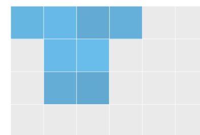
Fixed + Regressed
