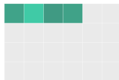
Fixed Variability
