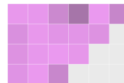
With Interaction
