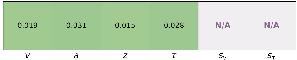
Calibration Error
