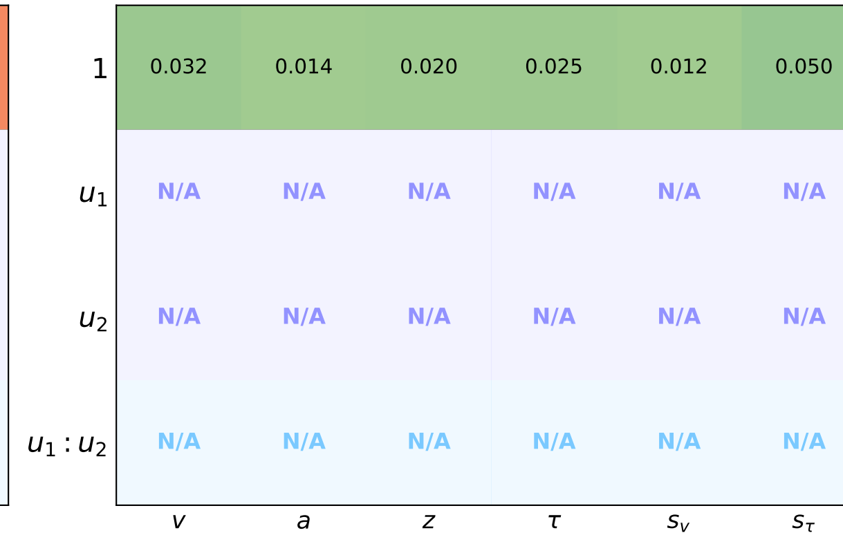
Calibration Error
