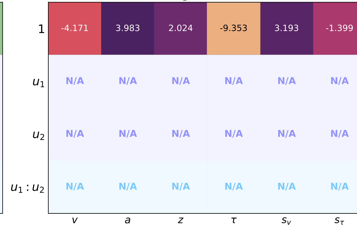
Log Gamma
