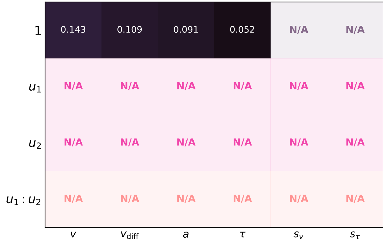
NRMSE
