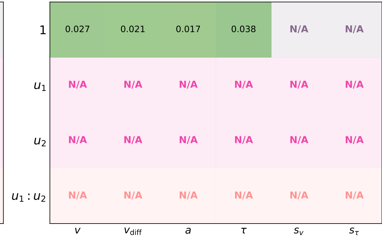
Calibration Error
