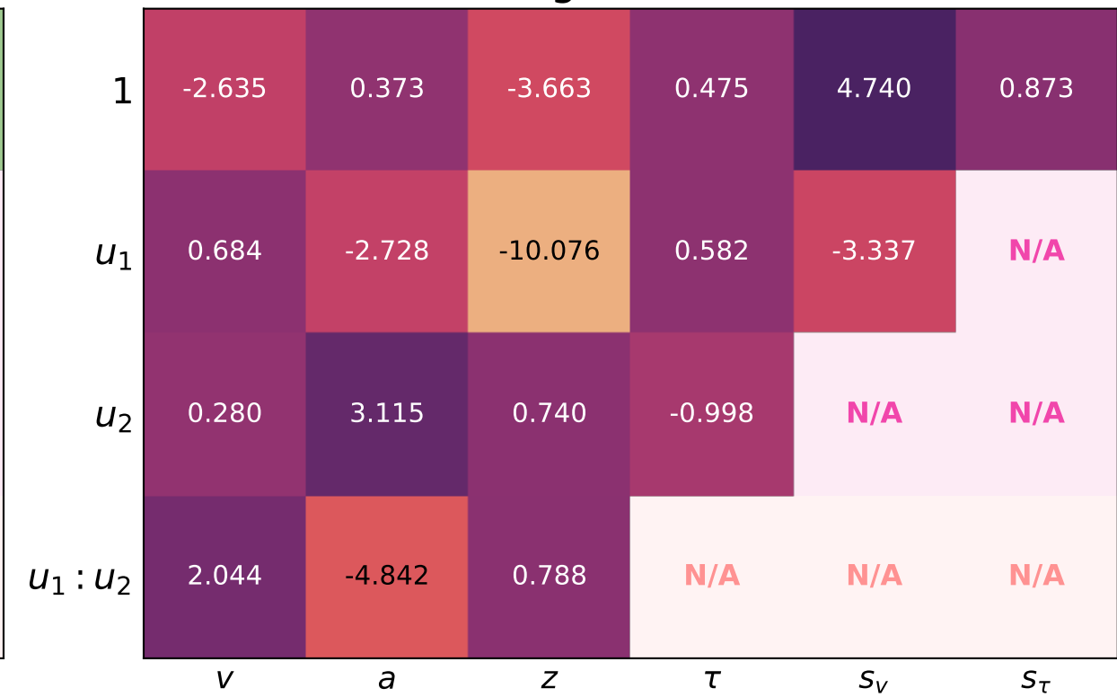
Log Gamma
