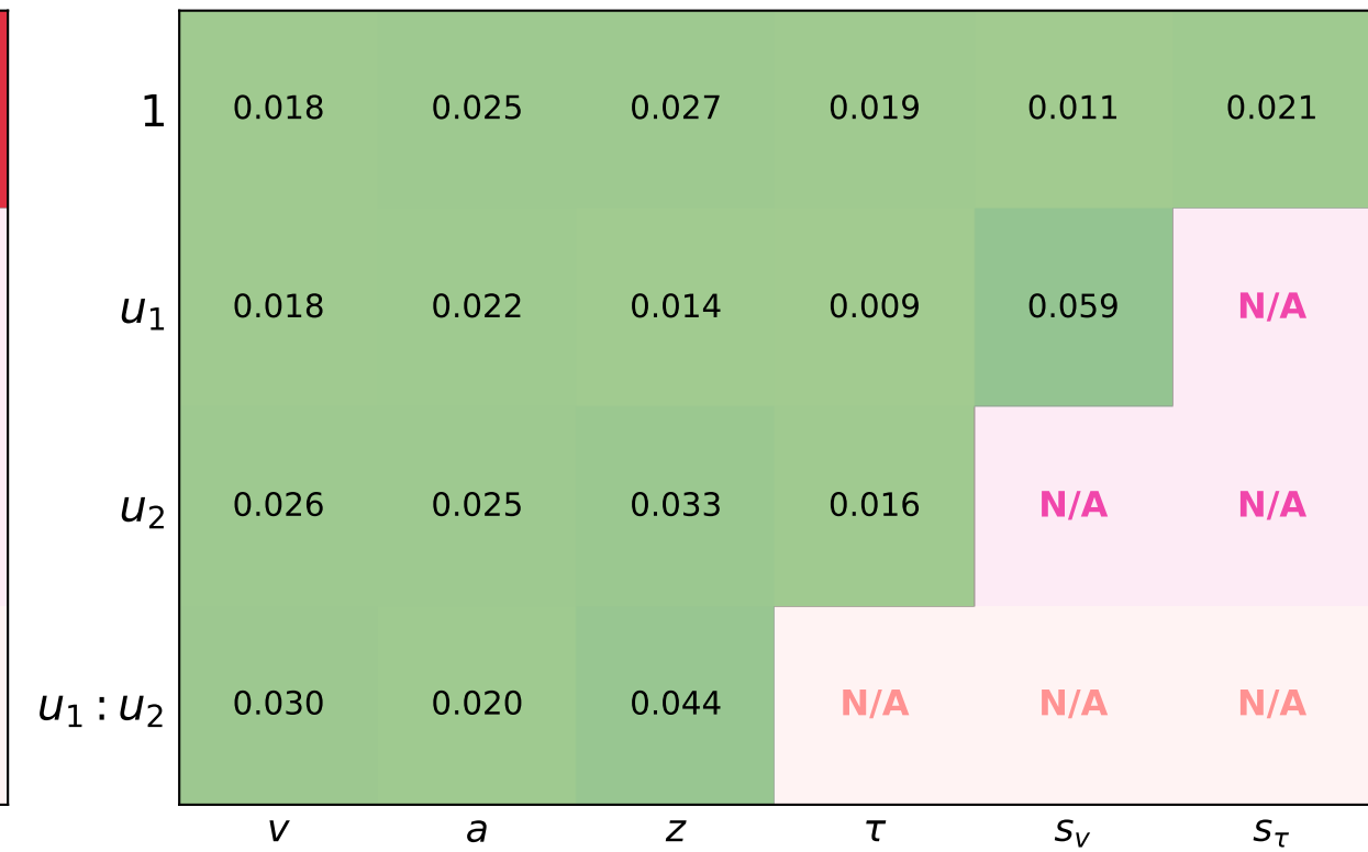
Calibration Error
