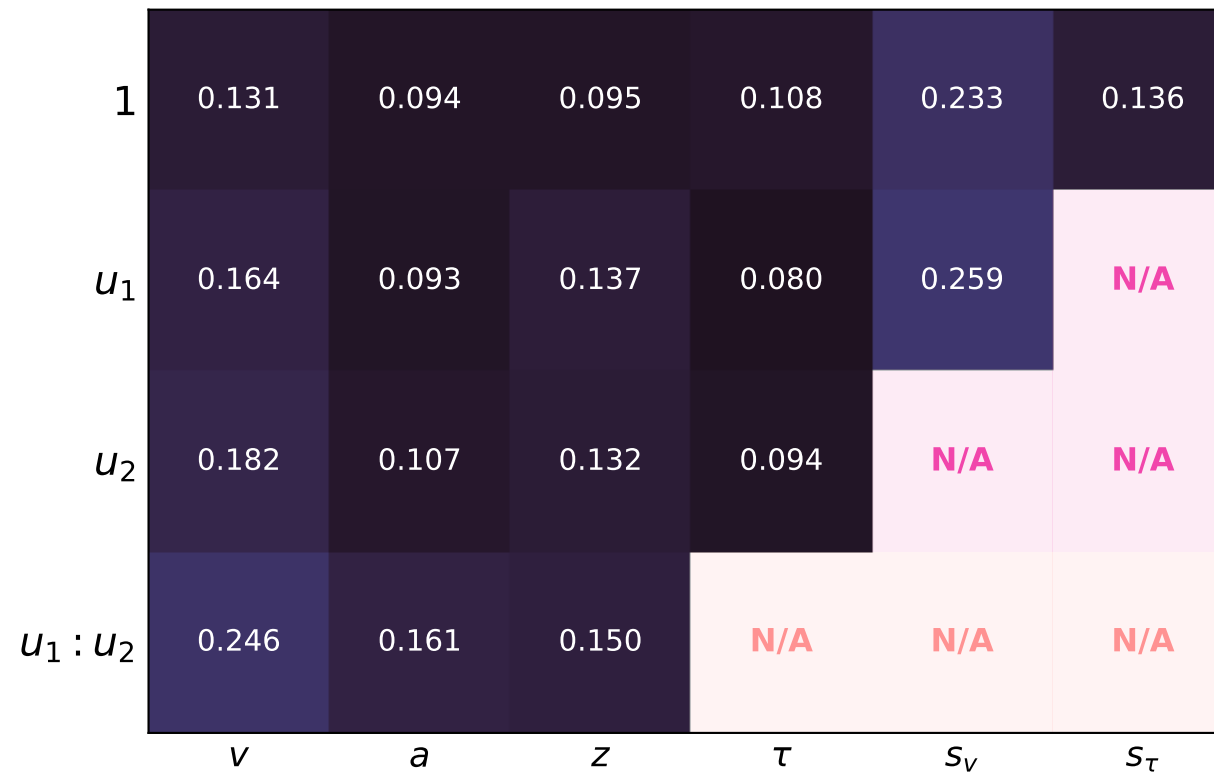
NRMSE
