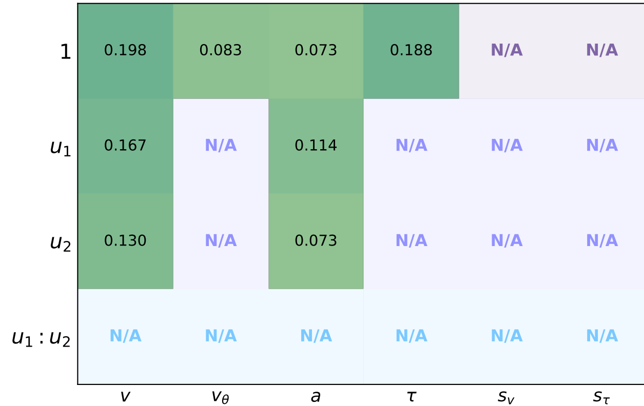
Calibration Error
