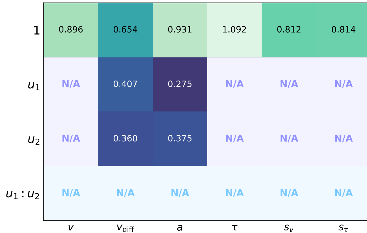
NRMSE
