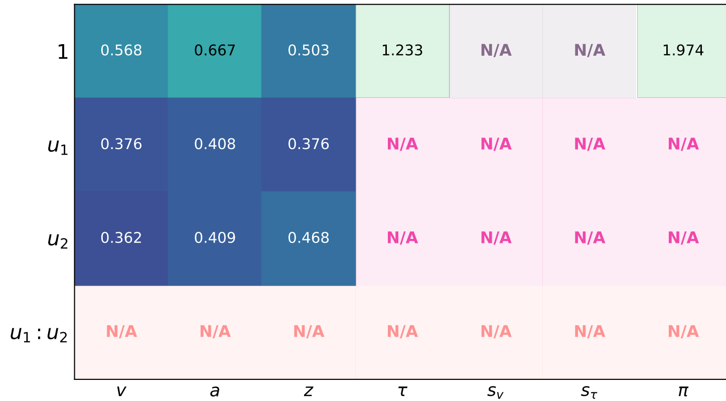
NRMSE
