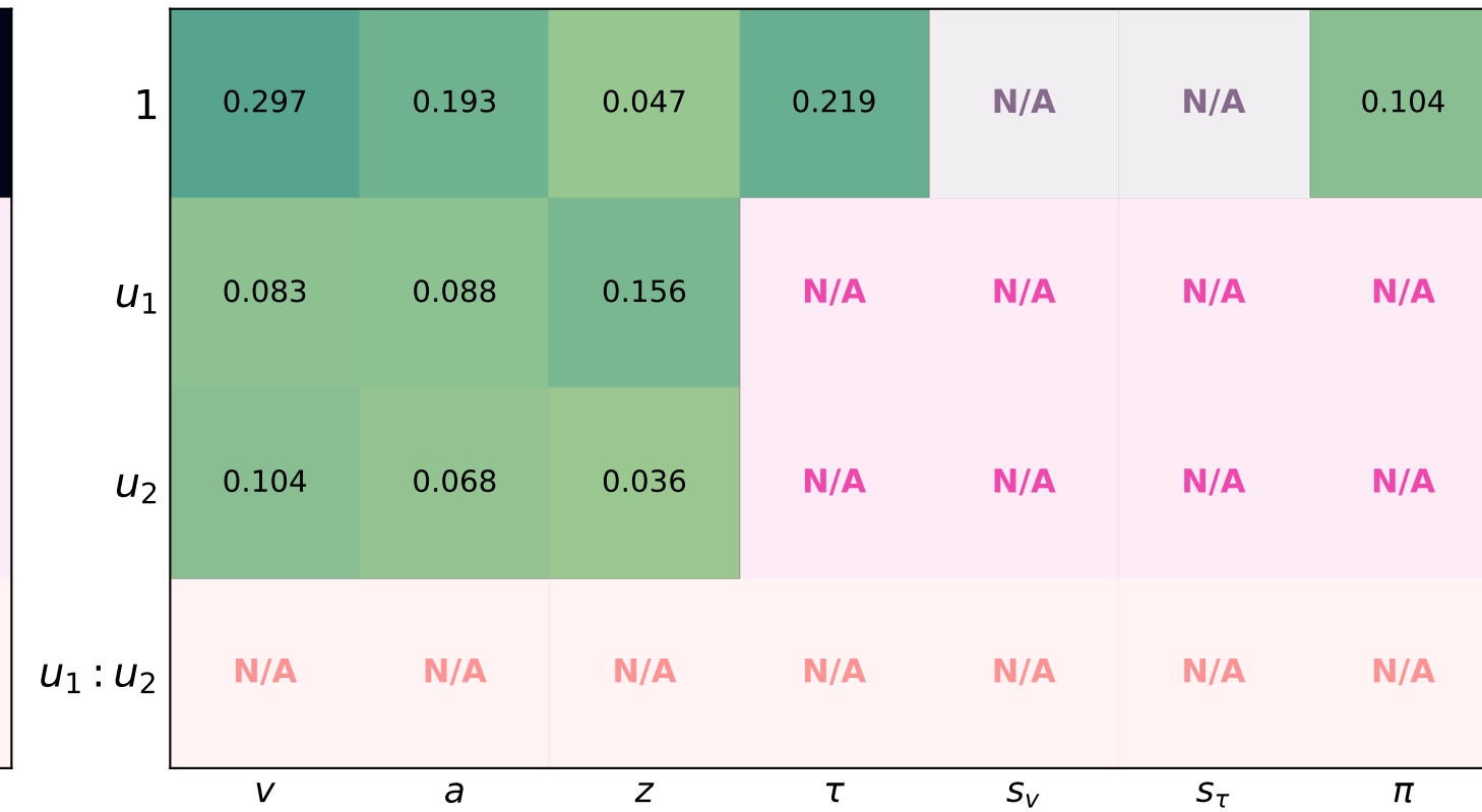
Calibration Error
