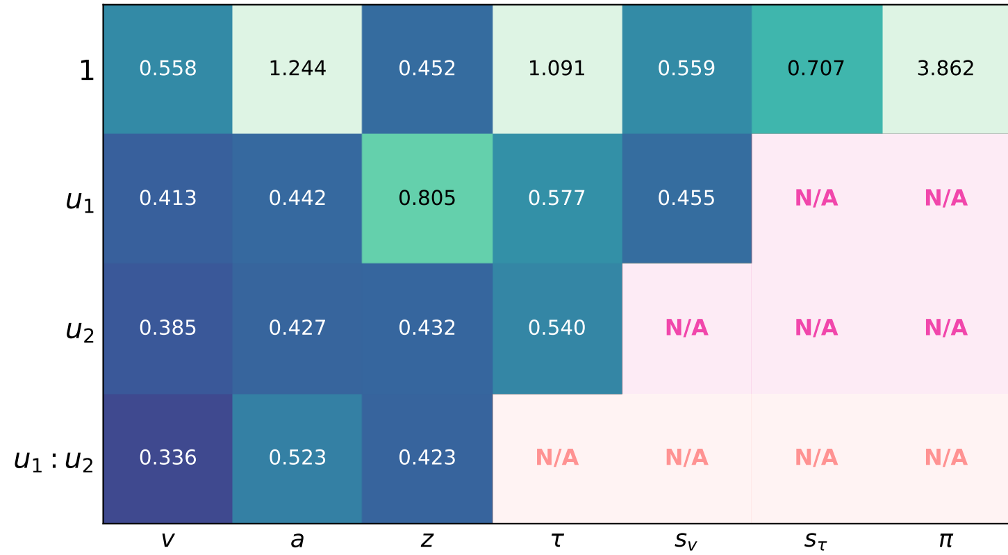
NRMSE
