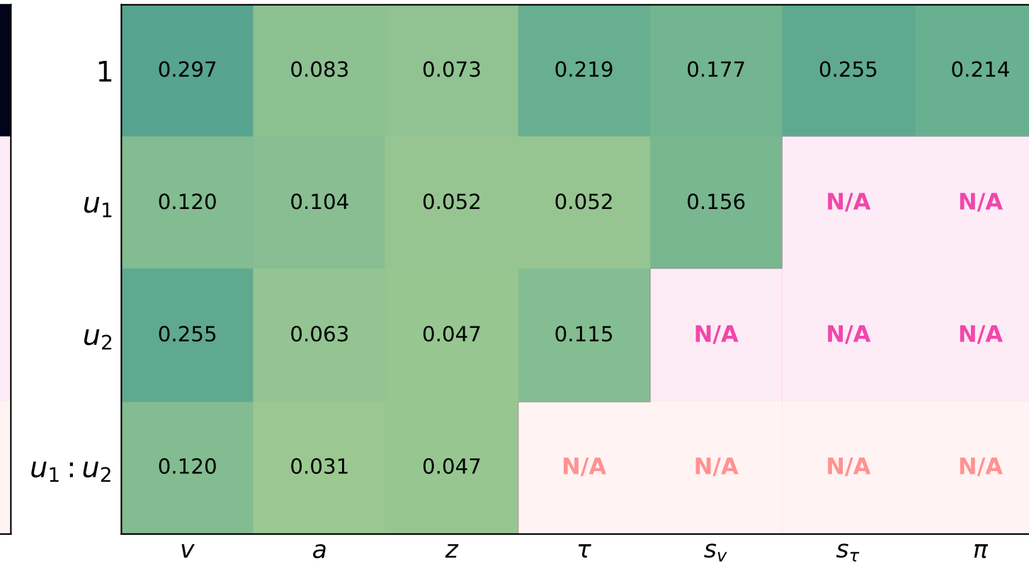
Calibration Error
