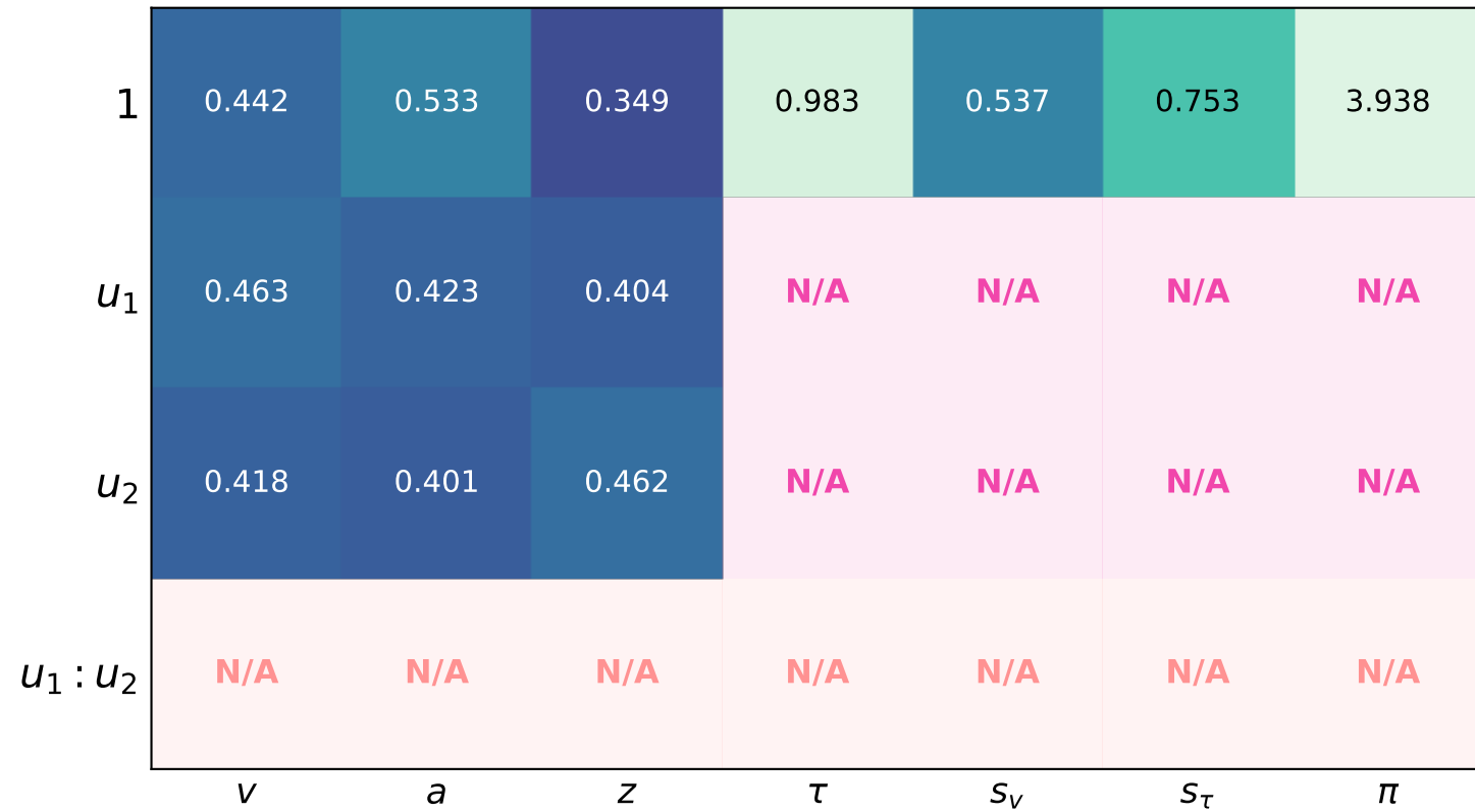
NRMSE
