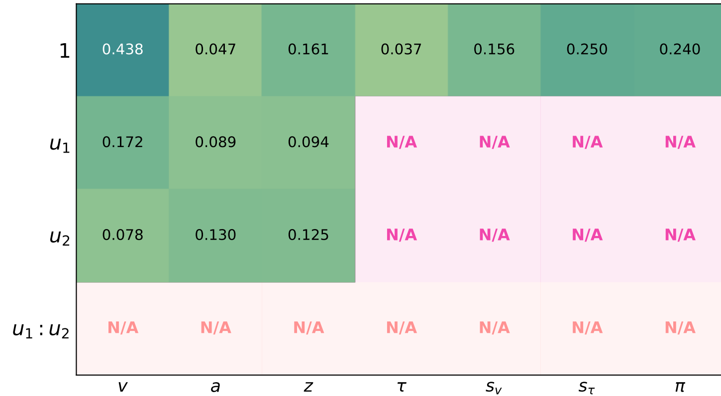
Calibration Error
