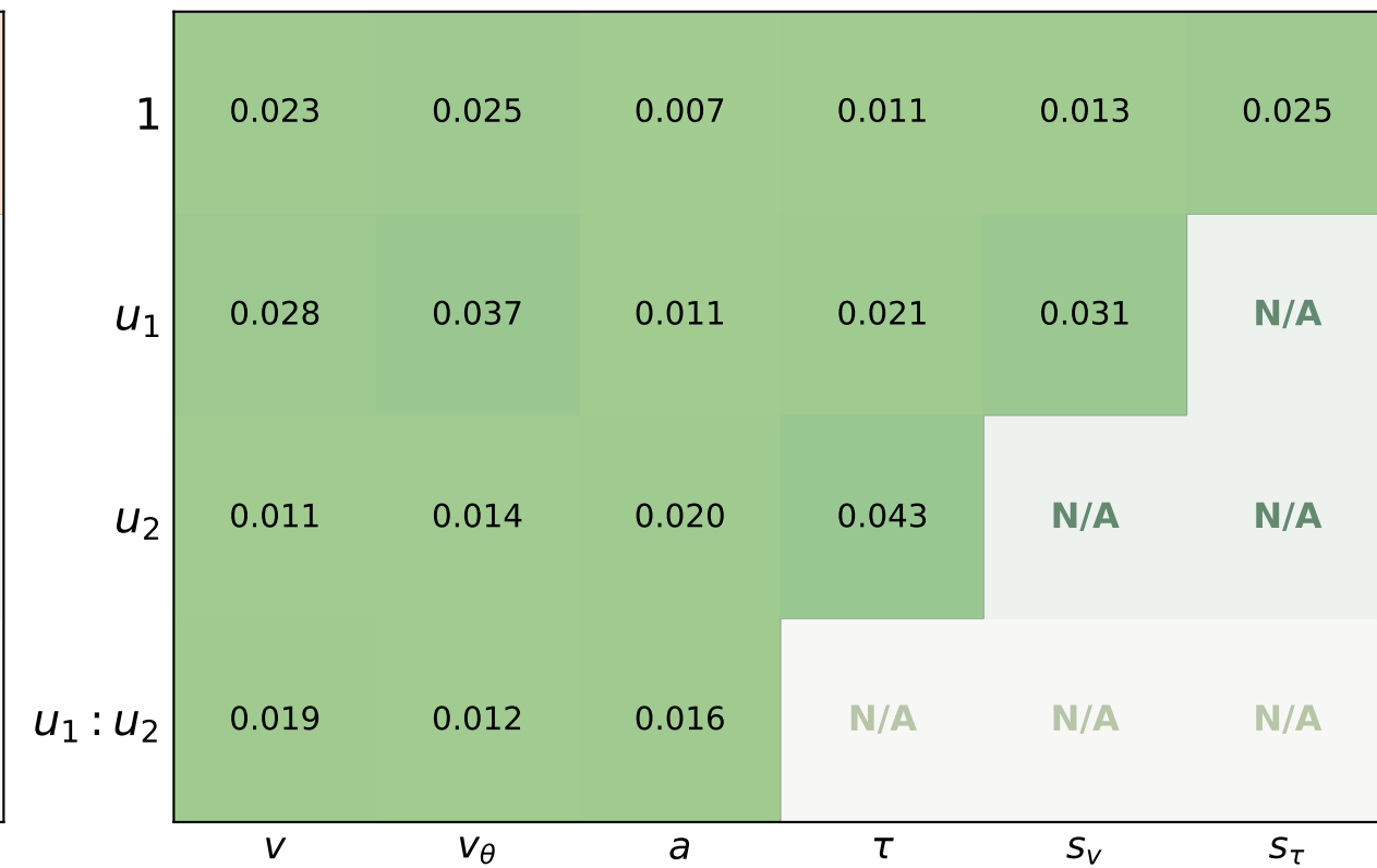
Calibration Error
