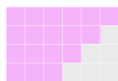
interaction
