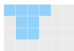
fixed_regressed
