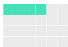
fixed
