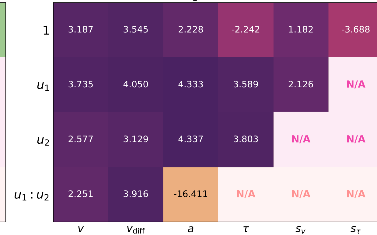
Log Gamma
