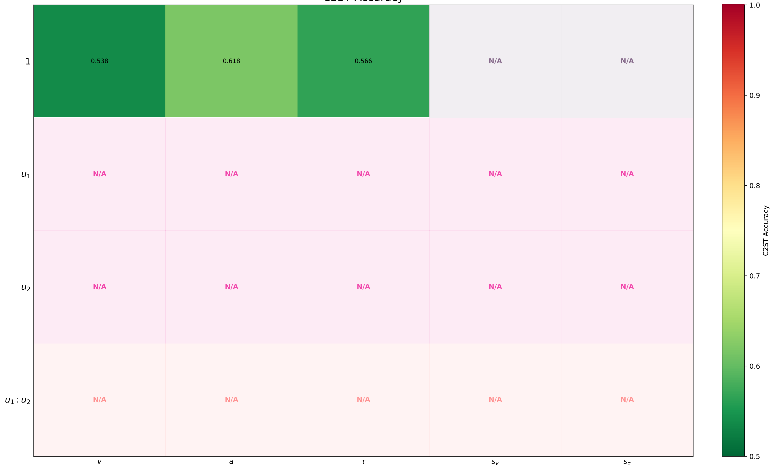
C2ST Accuracy
