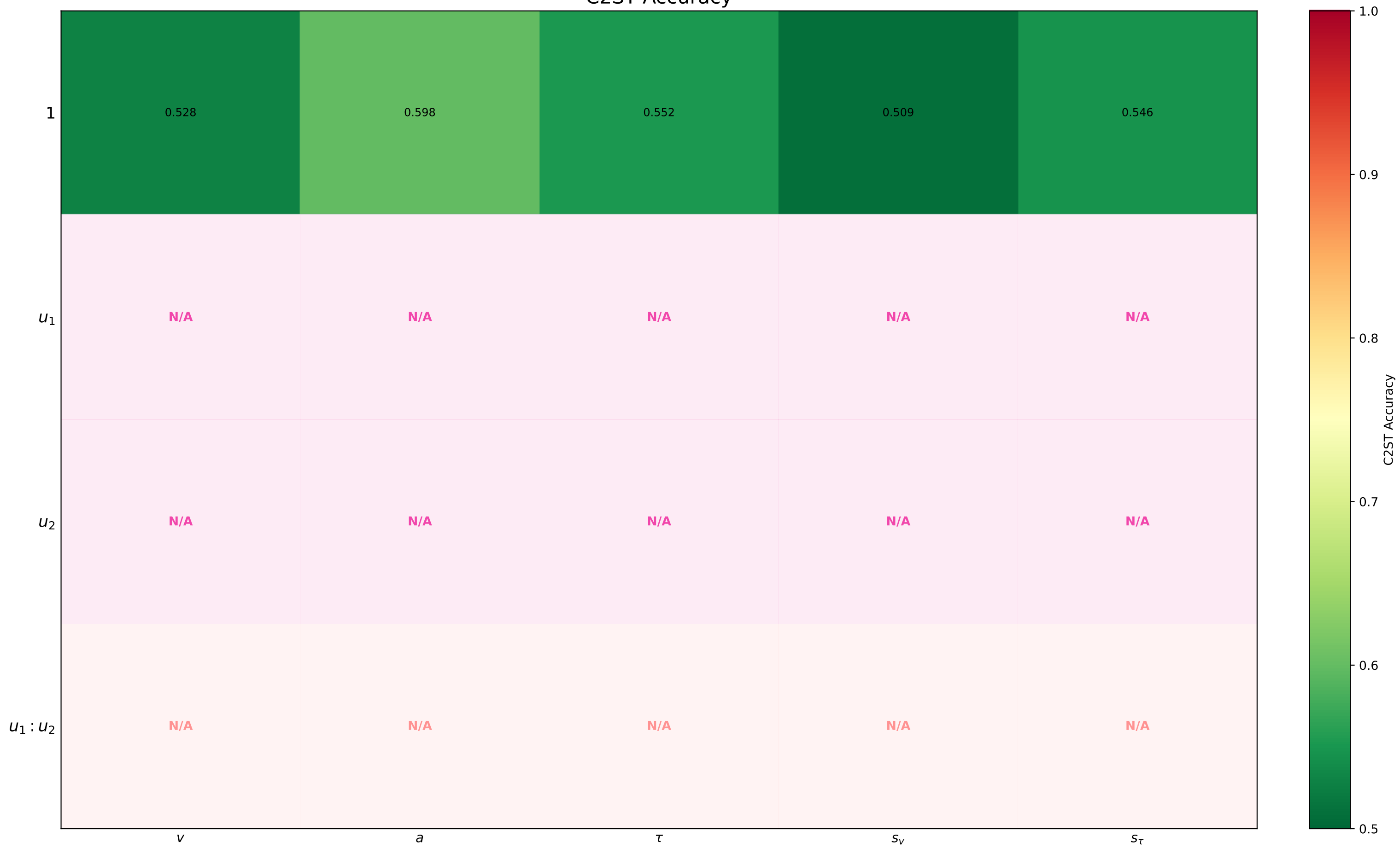
C2ST Accuracy
