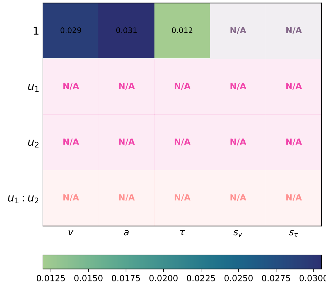
Calibration Error
