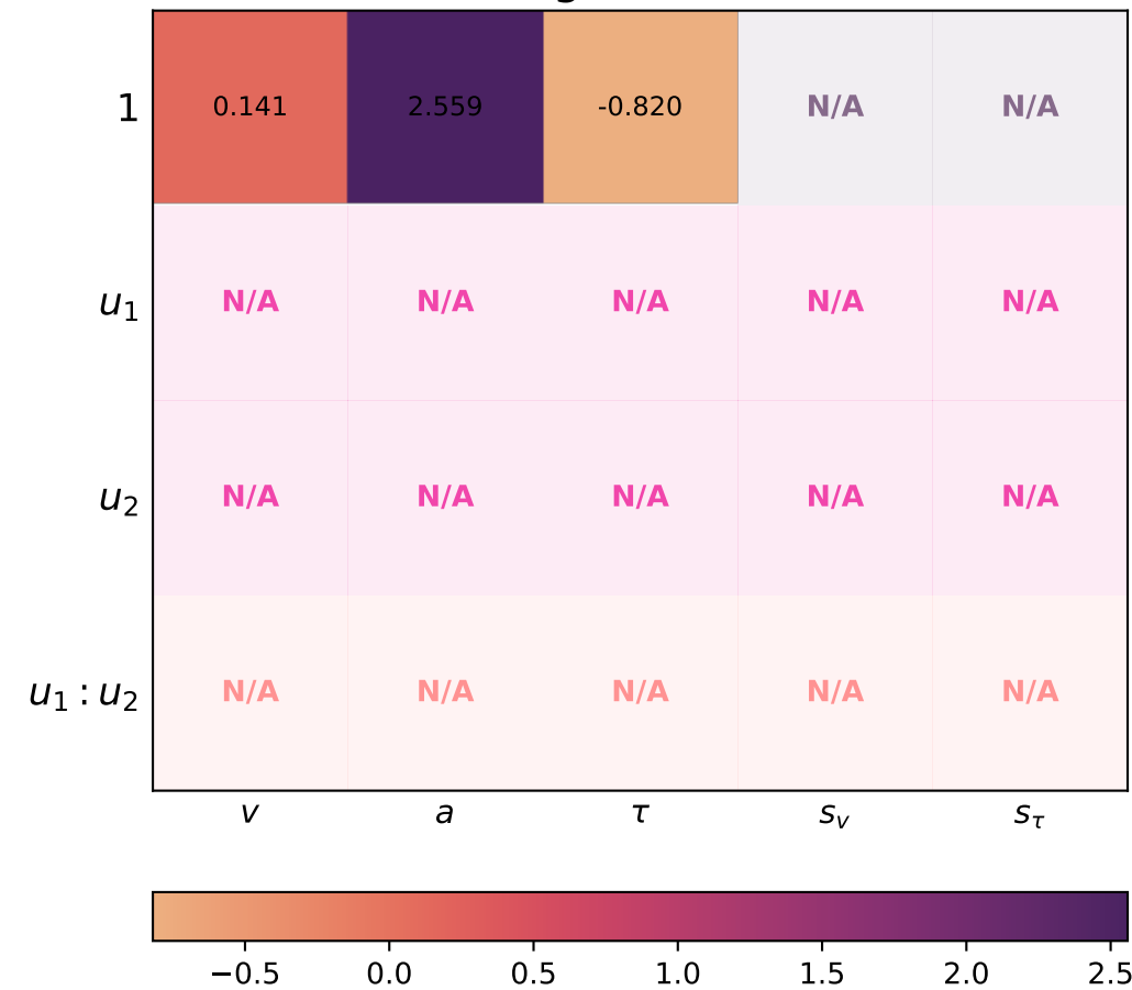
Log Gamma
