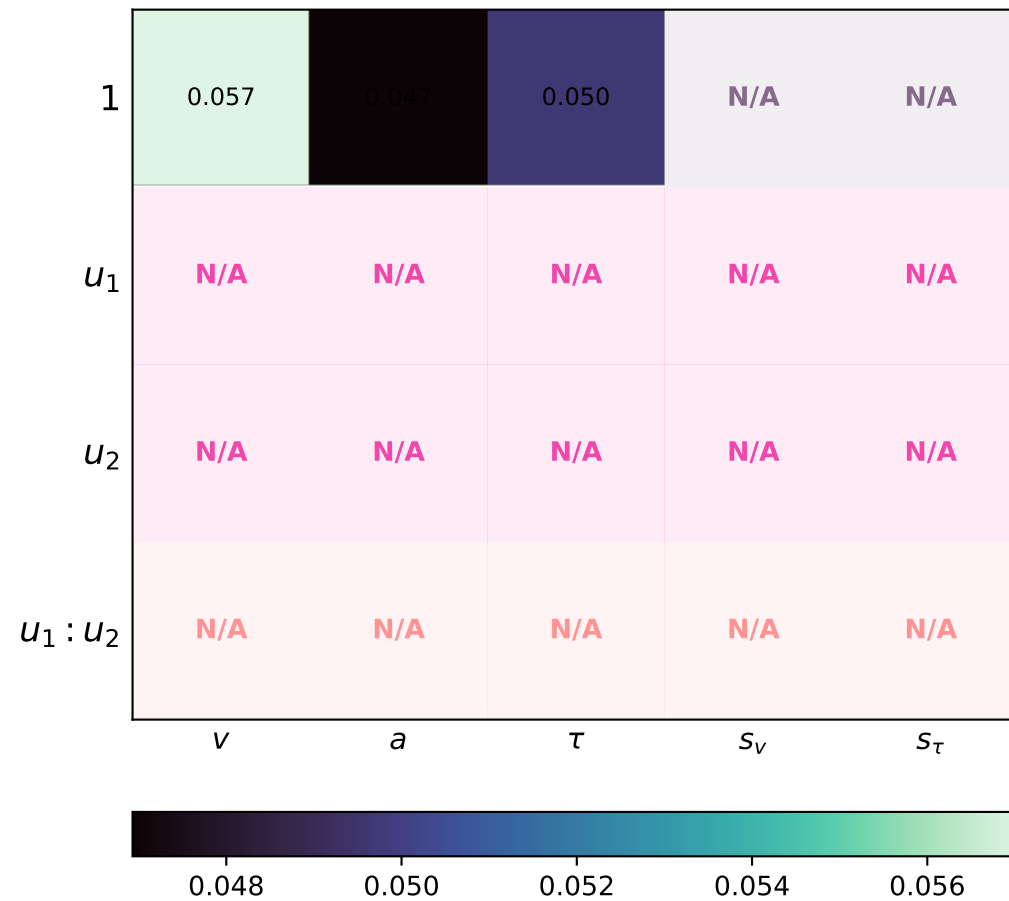
NRMSE
