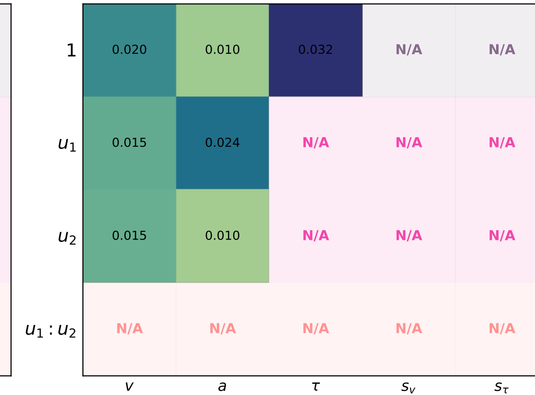
Calibration Error
