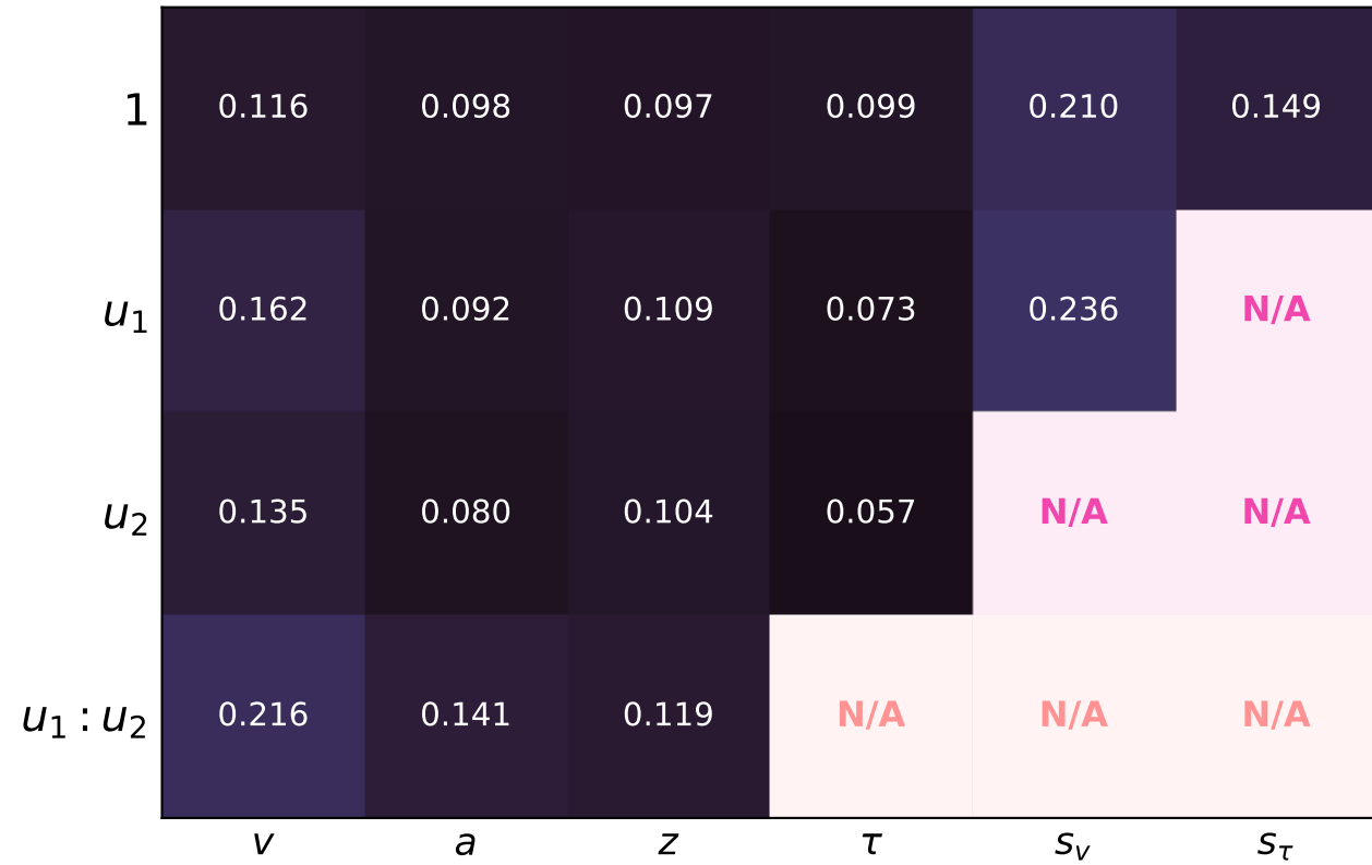
NRMSE
