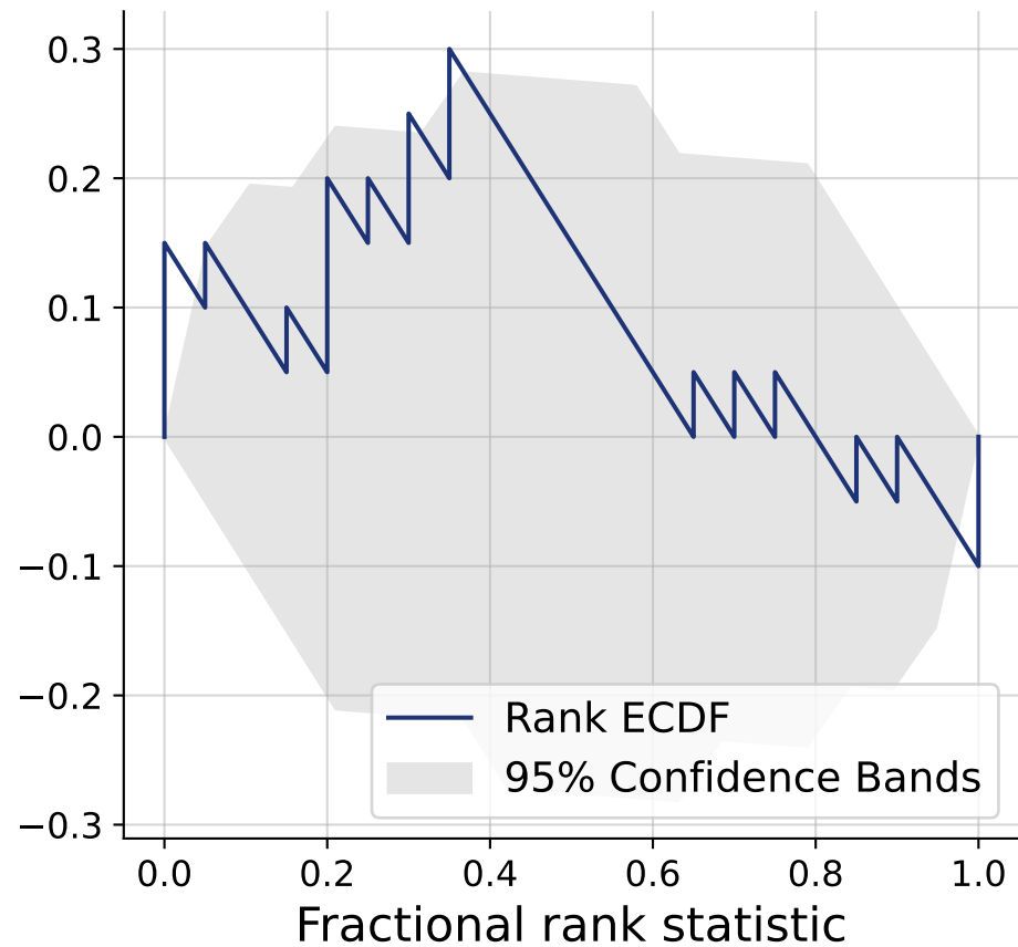
ECDF Difference
