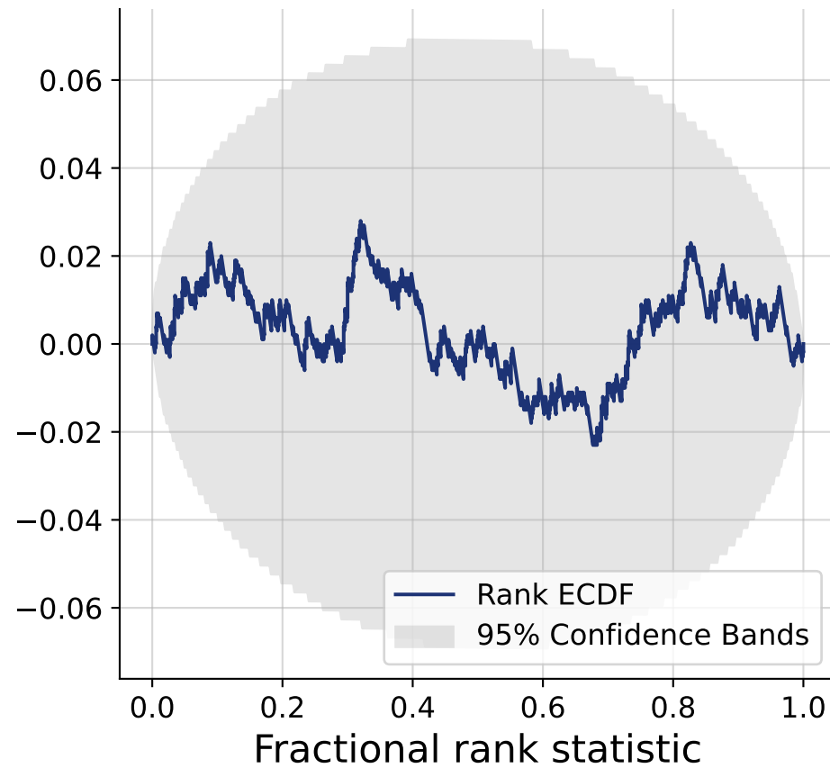
ECDF Difference
