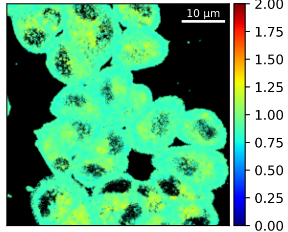
Estimates MLE \tau^{\text{mean}}
