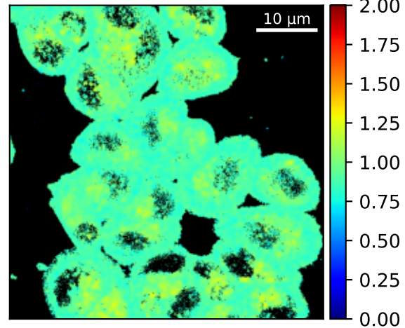
Estimates MLE \tau^{\text{mean}}
