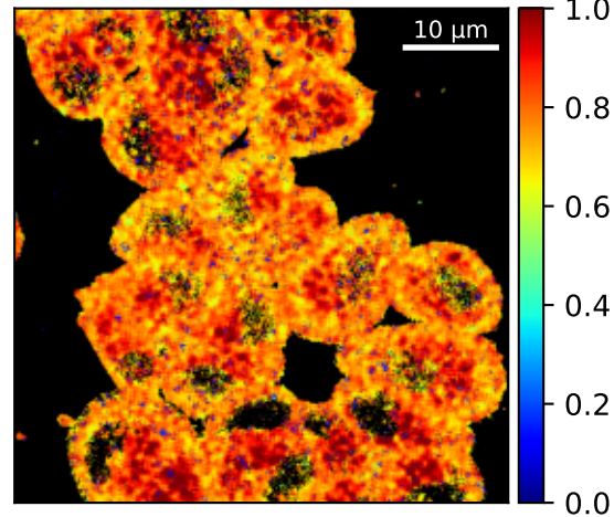
Estimates MLE \tau_1^L
