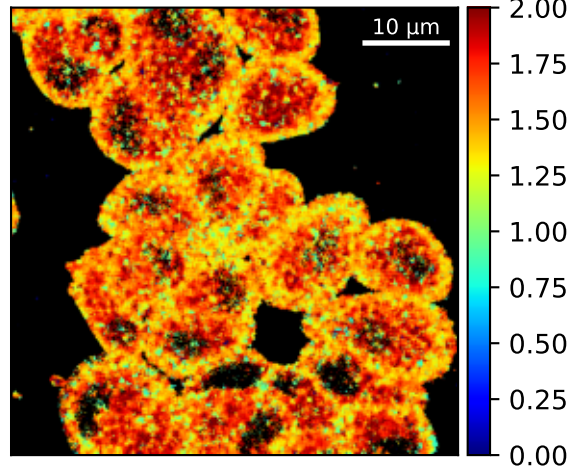
Estimates MLE \tau_2^L
