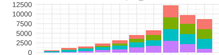
cathepsin_C
