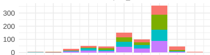
cathepsin_C
