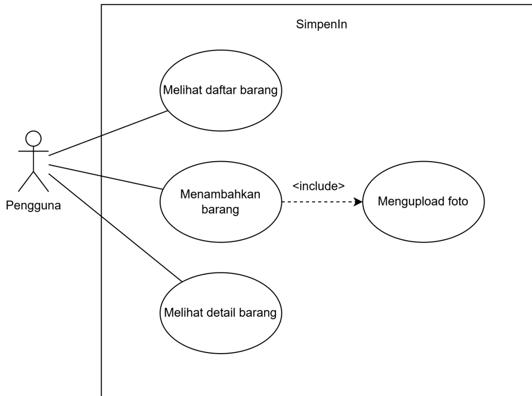
Gambar 1. Use Case Diagram SimpenIn
