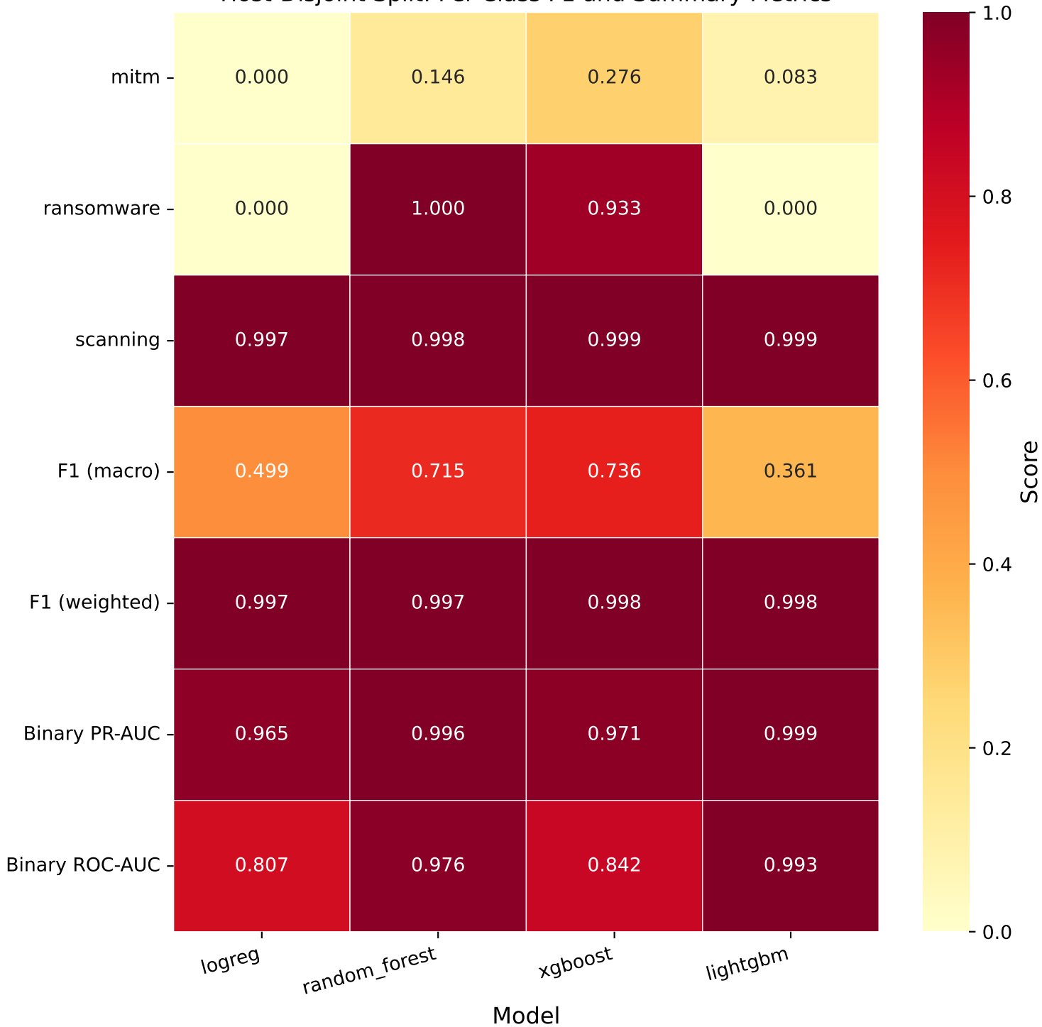
Host-Disjoint Split: Per-Class F1 and Summary Metrics
