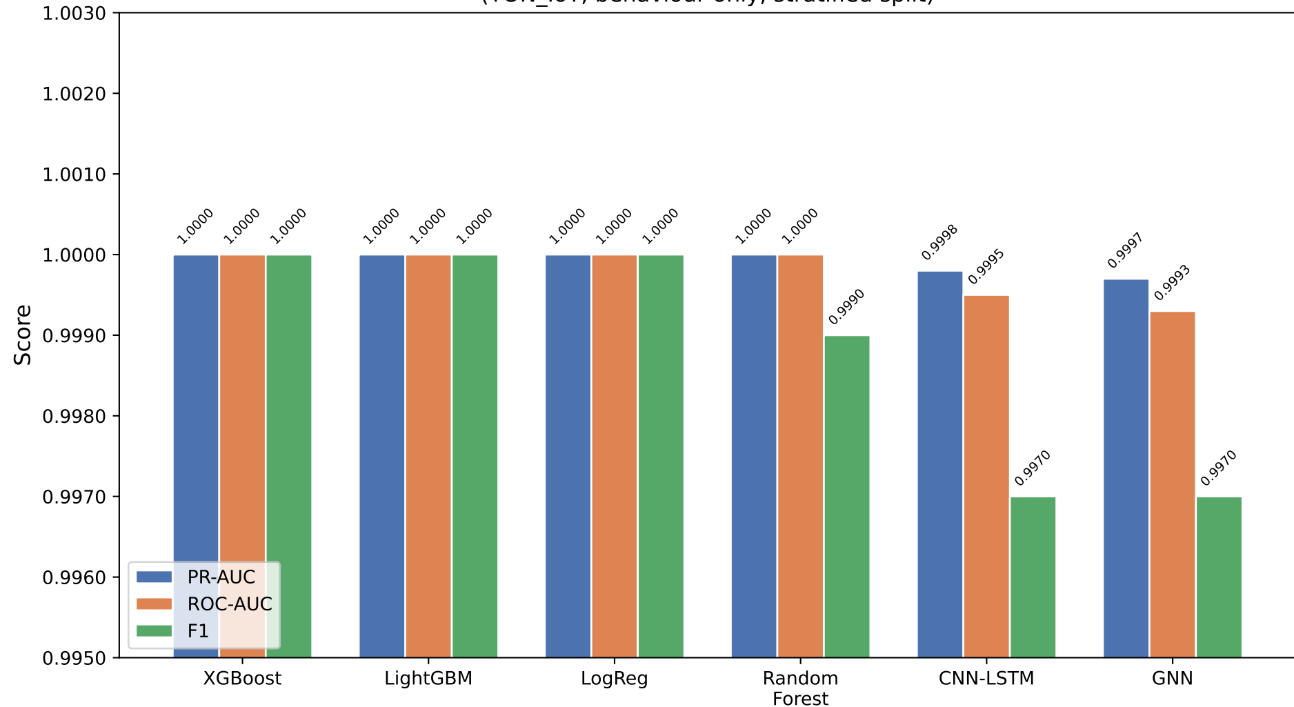
Binary Detection Performance Across All Model Families (TON_IoT, behaviour-only, stratified split)
