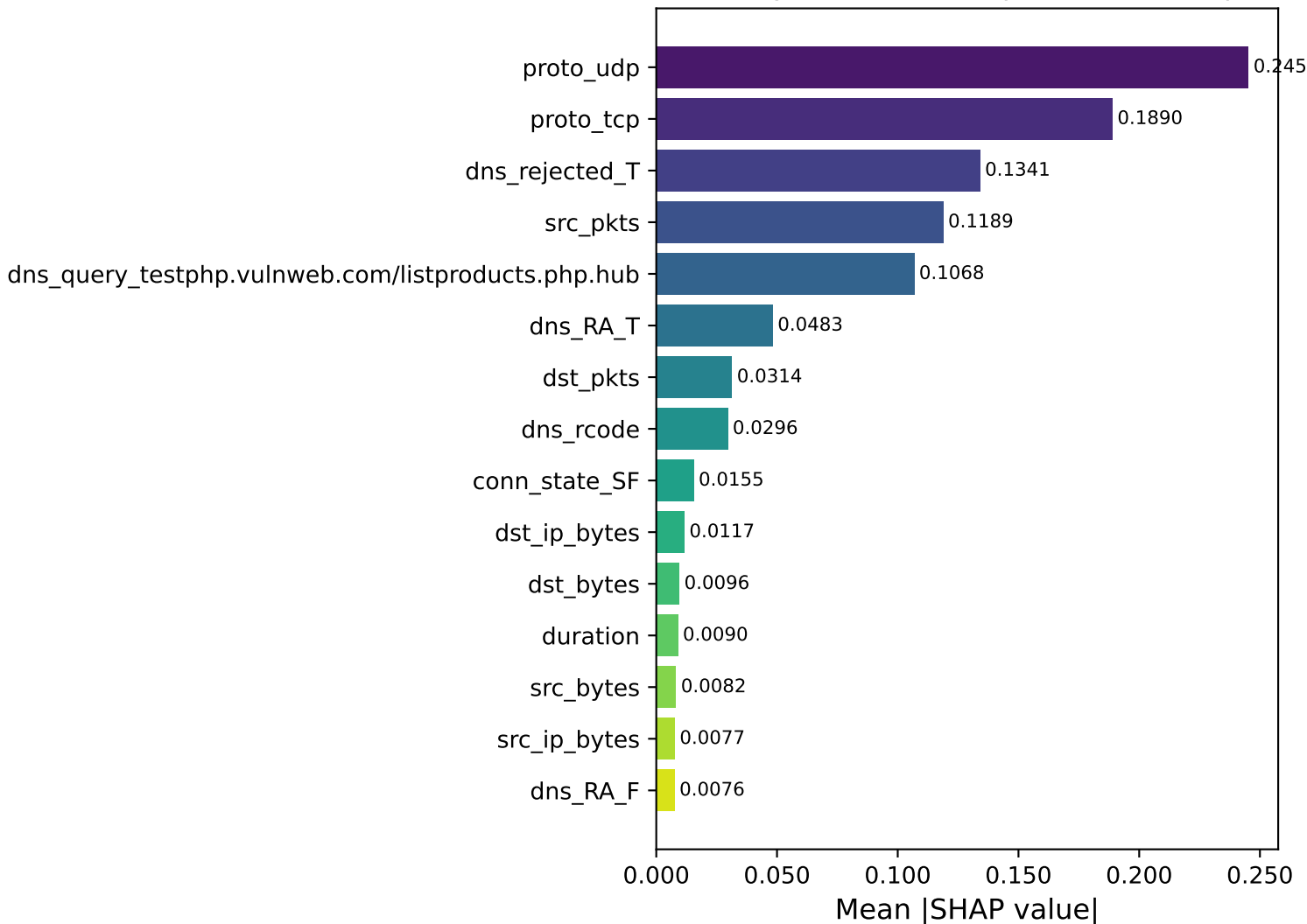
XGBoost Binary Detection -- Top 15 Feature Importances
