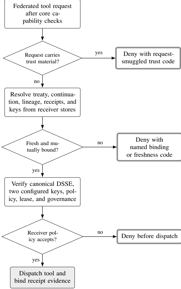
Figure 2: Receiver-side pre-dispatch admission. Trust material flows from receiver-owned stores, not from the request. Every denial terminal precedes the tool boundary.
