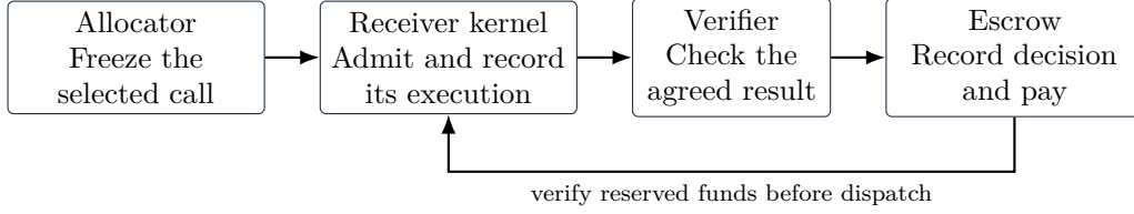
Figure 2: Each authority checks records referring to the same call. The receiver checks local permission and reserved funds before execution. Its evidence feeds the verifier, whose recorded decision governs payment.
