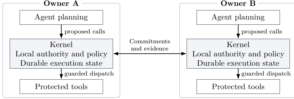
Figure 1: Local enforcement within a distributed program. Each owner controls its kernel’s authority and protected state. The interdomain arrow denotes signed records exchanged through the protocol, independently of their transport.
