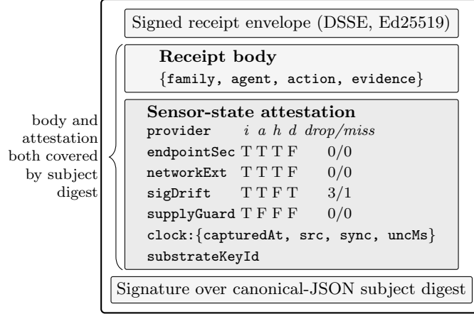
Figure 1: Sensor-state attestation traveling with every signed receipt. The substrate’s signing key covers both the body bytes and the per-sensor health record, so the verifier evaluates substrate posture as part of admission, not as a side channel. Flag column headings: installed , active , healthy , degraded .
