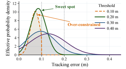
Fig. 7: Precision–stability sweep over \delta_{\text{term}} \in \{0.1, 0.2, 0.3, 0.4\} m.
