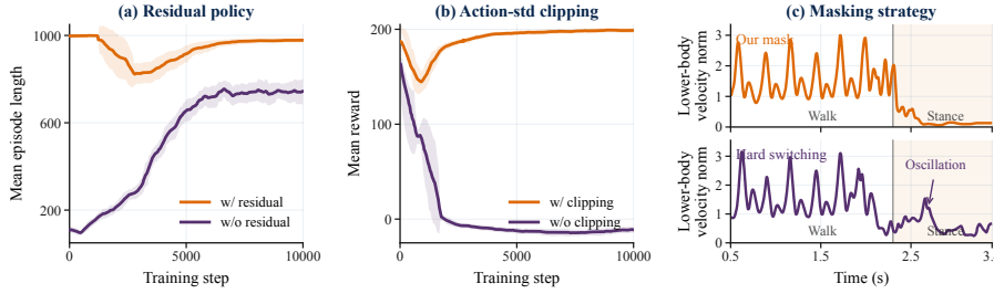
Fig. 6: Unified-control ablations. (a) Asymmetric base+residual converges, unlike end-to-end 29-DoF learning. (b) Residual action-std clipping prevents late collapse. (c) Masking reduces walk→stance discontinuities.
