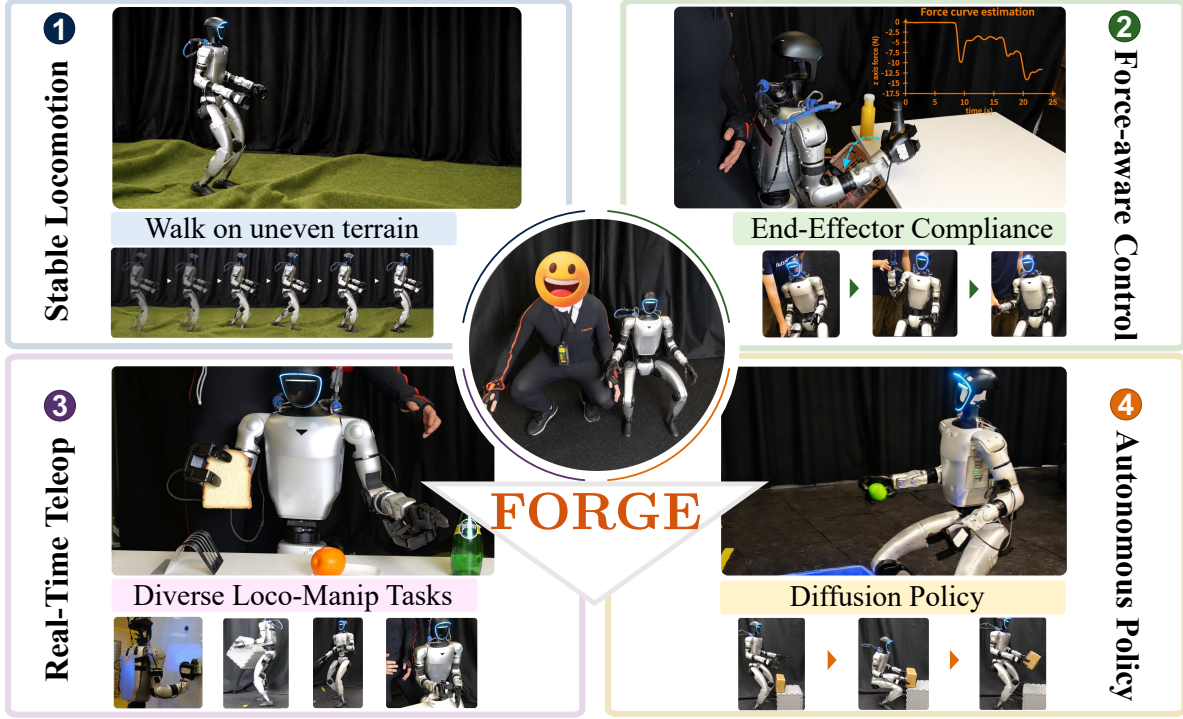
Fig. 1: FORGE enables efficient humanoid loco-manipulation via multi-granularity control: velocity navigation, foot placement, single-/dual-arm end-effector tracking, and force-conditioned contact adaptation.
