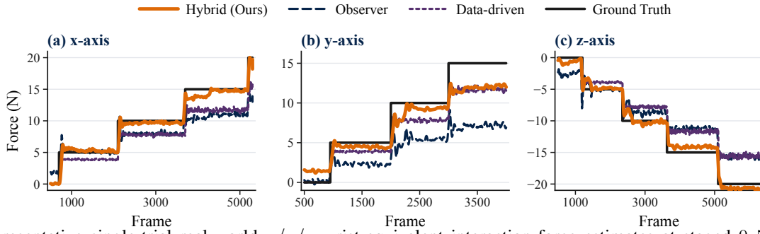
Fig. 8: Representative single-trial real-world x/y/z wrist-equivalent interaction-force estimates at staged 0, 5, 10, 15, 20 N loads. Each load is repeated 10 times with digitally synchronized force-gauge references; the gauge is used only for evaluation and is not an estimator input.
