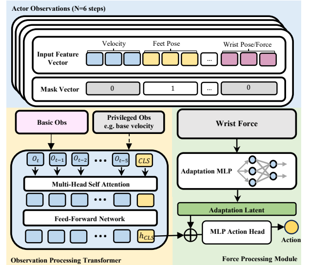
Fig. 3: Actor architecture. Solid deployment paths use only the masked observable history. “Wrist Force” denotes the observer-derived residual history, not a force/torque-sensor reading or simulator force. The adaptation decoder’s 6-D correction refines the observer at deployment; the dashed privileged quantities supply training targets only. produces the reachable distributions in Fig. 4; the actor observes wrist targets rather than the sampled joints and resolves whole-body IK implicitly.
