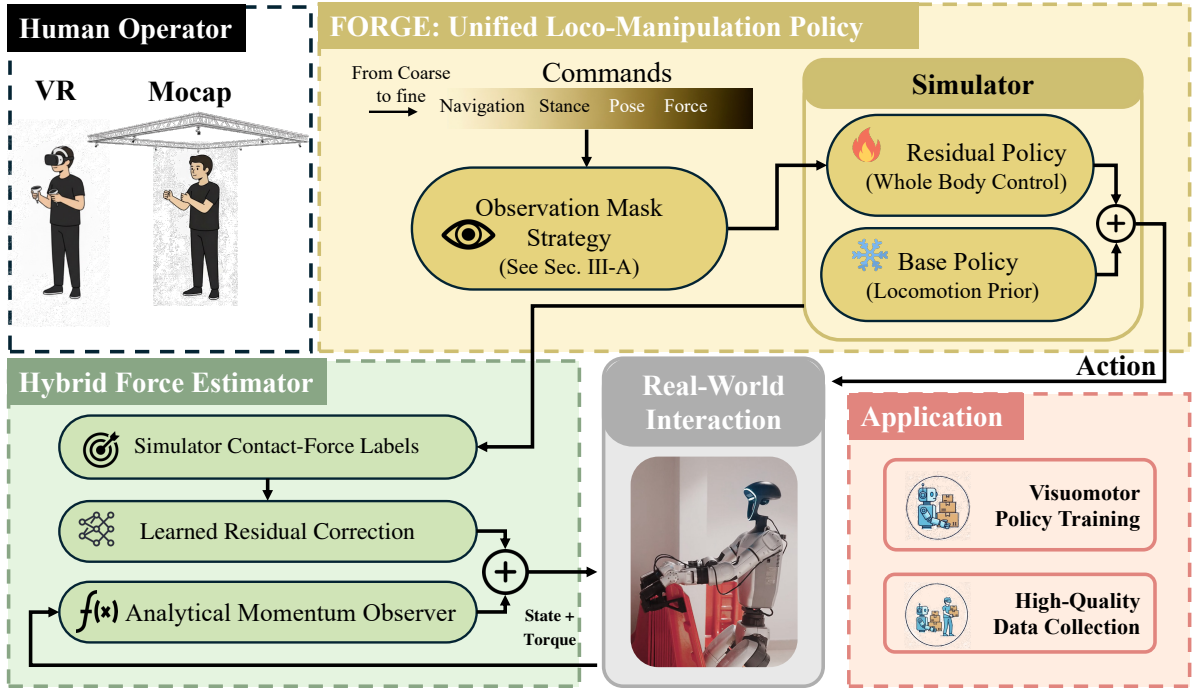
Fig. 2: Overall pipeline of FORGE. The framework has three components: multi-granularity control over navigation, stance, pose, and optional force-conditioning inputs; a physics-informed hybrid force estimator and virtual-target contact-adaptation loop; and asymmetric residual actions anchored on a frozen locomotion prior. Policy training uses sparse task-space commands rather than full-body human motion references.
