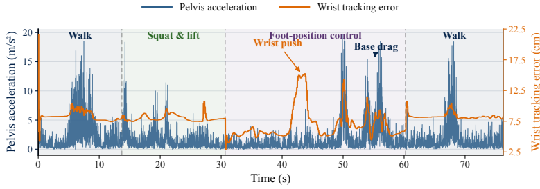
Fig. 10: Pelvis acceleration and wrist-error traces across walking, squat/lift, and foot-position control under wrist-push and base-drag perturbations, with transient deviations followed by recovery.
