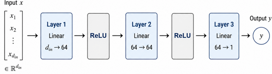
Fig. 3: Structure of one cost network. The input is a fixed-length feature vector for one candidate, and ReLU follows each of the two 64-unit hidden layers. The output is one pair-centred cost score. A decision evaluates every candidate with the same network and takes the argmin. The proposal and acceptance policies share this structure and differ only in input dimension, 21 and 16 respectively.
