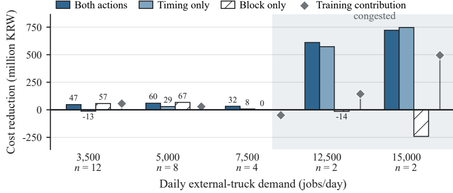
Fig. 6: Cost reduction by demand level, decomposed by action range. The values are those of Table 4, in million KRW (1 bn = 1,000 m). All five demand levels share one axis, and the shaded band marks the two congested levels. Because those two are more than ten times larger than the rest, the value is printed next to each short bar. The number of days observed appears as n under each tick. Bars measure a restricted policy against no reallocation. The diamond is not a fourth action: it is the trained model minus the untrained one—the training contribution, that is, the last column of Table 4—and carries a different mark for that reason. Moving from the non-congested to the congested regime, arrival-time adjustment and the training contribution both grow sharply, whereas block-only reallocation turns negative.
