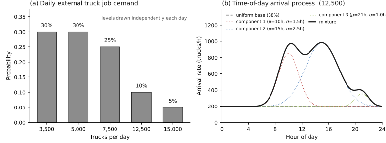
Fig. 2: External truck job demand. (a) The five daily demand levels and the probability with which each is drawn, independently for each day. (b) The arrival process at one congested level, with the uniform base and the three Gaussian components shown separately. The literature supports the demand magnitudes and the fact that arrivals are far from uniform over the day; the shape of the mixture is a construction of this study.
