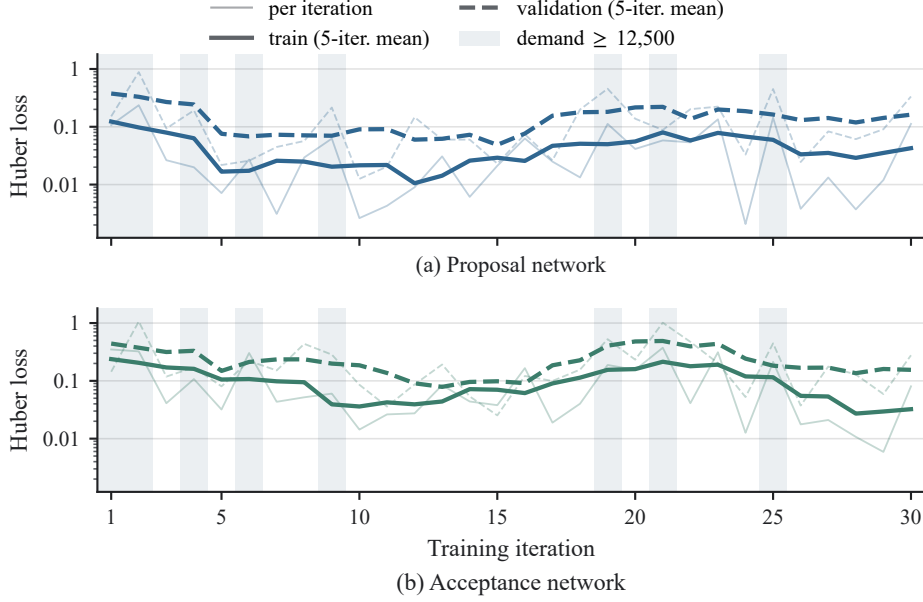
Fig. 3: Training and validation loss over the 30 iterations, with the per-iteration value drawn faintly beneath a five-iteration mean; the vertical axis is logarithmic. Shading marks the iterations whose demand was drawn at 12,500 or above, so much of the visible fluctuation follows that draw rather than the fit. Exploration decreased linearly from 0.50 to 0.05.
