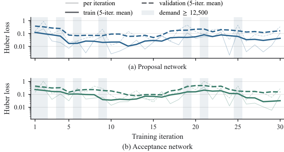
Fig. 3: Training and validation loss over the 30 iterations; the faint line is the per-iteration value beneath a five-iteration mean, and the vertical axis is logarithmic. Shading marks the iterations whose demand level was 12,500 or above, so much of the visible fluctuation follows that draw rather than the fit. Exploration fell linearly from 0.50 to 0.05.
