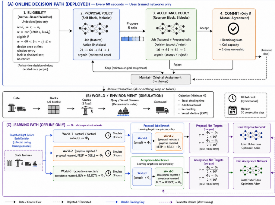
Fig. 1: The proposed architecture. (a) Every 60 s the operational path checks eligibility, proposal, acceptance, and commitment; one-sided consent or a capacity failure keeps the original assignment. (b) The discrete-event environment links gate, blocks, yard cranes, and vessel operations to compute the cost \Phi . (c) Offline learning compares up to three worlds from the same state and random stream over 3 h and labels the two cost networks.
