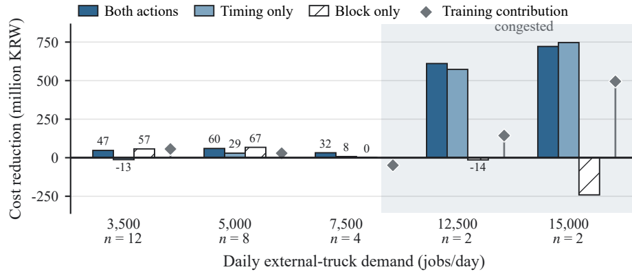
Fig. 2: Cost reduction by demand level, decomposed by action range, in million KRW. The shaded band marks the two congested levels; values are printed beside the short bars and n is the number of days observed. Bars compare a restricted policy with no reallocation; the diamond is the learned policy minus the first-iteration model. The split between the two action types is specific to this demand mix.
