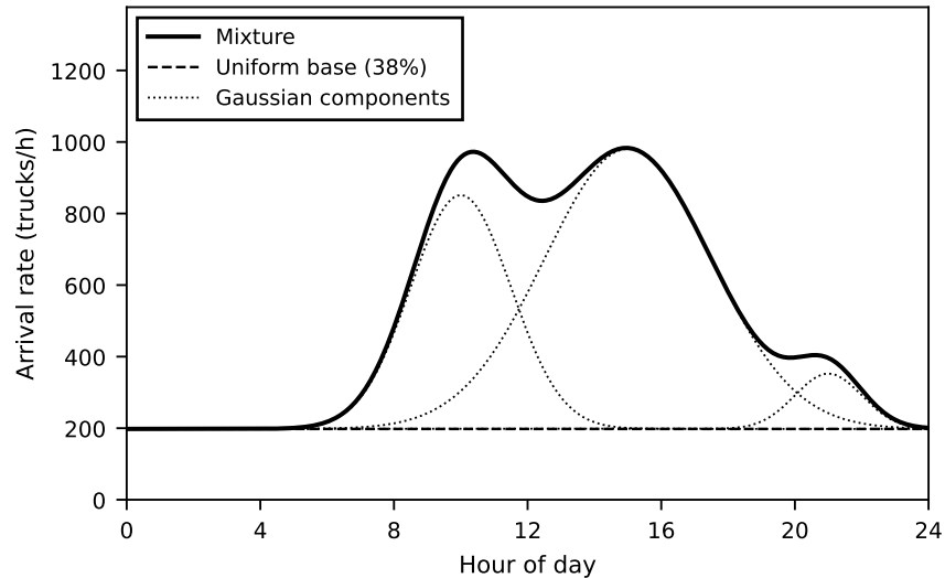
(b) Arrival process at 12,500 trucks/day
