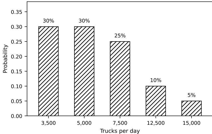
(a) Daily external truck job demand
