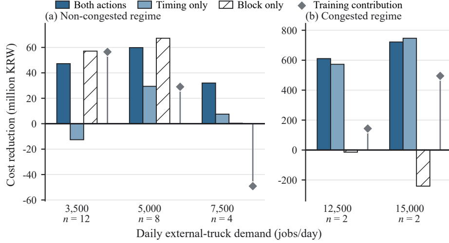
Fig. 5: Cost reduction by demand level, decomposed by action range. The values are those of Table 4, in million KRW (1 bn = 1,000 m). The vertical axis is split by demand because the two congested levels are more than ten times larger than the rest: (a) 3,500–7,500 and (b) 12,500–15,000 jobs per day, with the number of days observed printed as n under each tick. Bars measure a restricted policy against no reallocation. The diamond is not a fourth action: it is the trained model minus the untrained one—the training contribution, that is, the last column of Table 4—and carries a different mark for that reason. Moving from the non-congested to the congested regime, arrival-time adjustment and the training contribution both grow sharply, whereas block-only reallocation turns negative.
